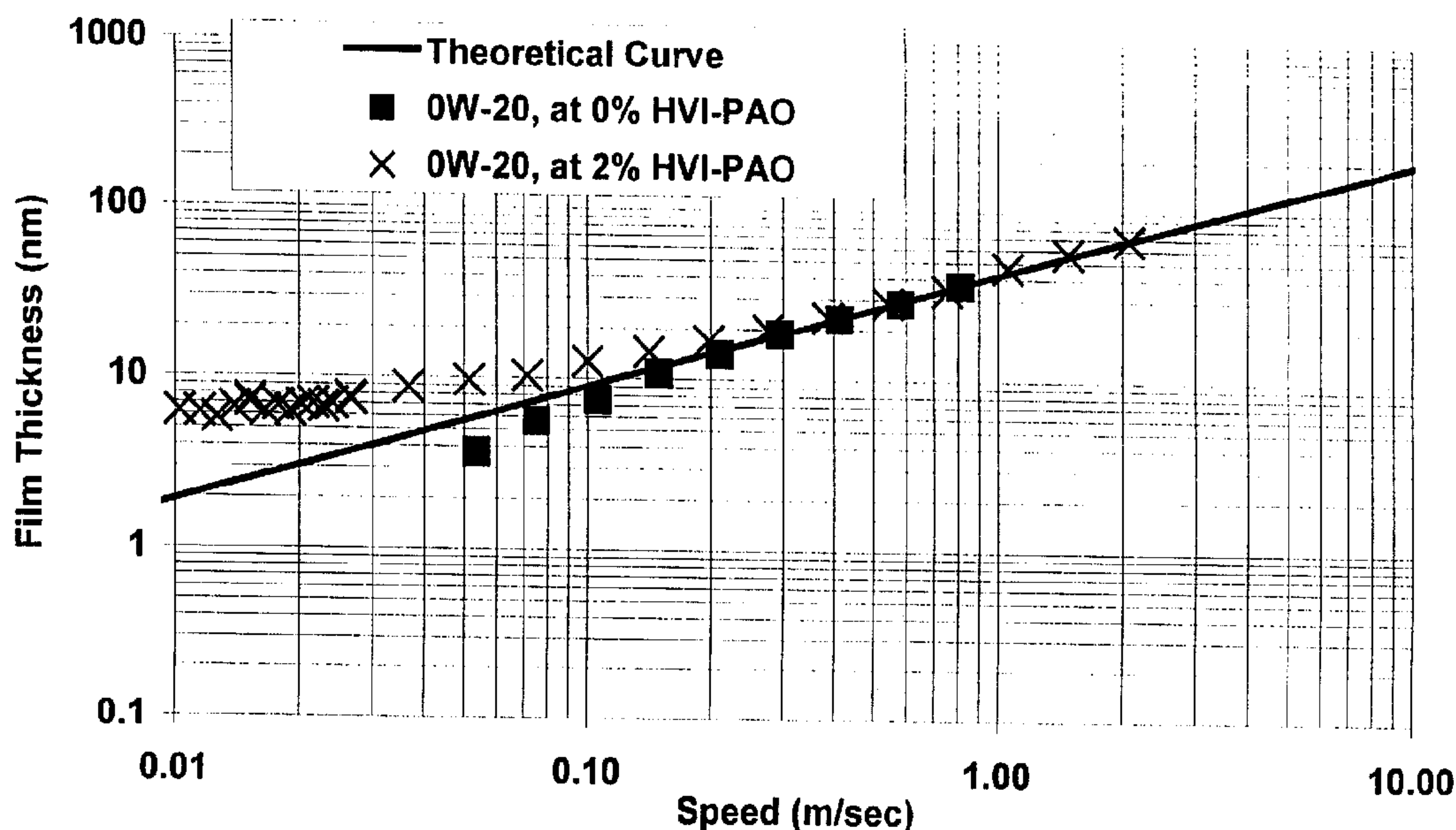
Film Thickness Performance of HVI-PAO Base Oil
