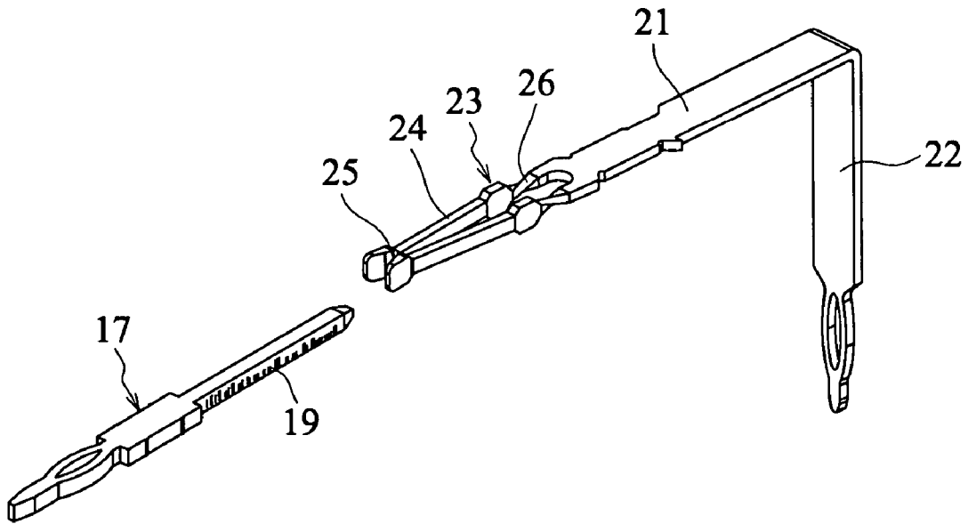
FIG. 5 (Prior Art)
