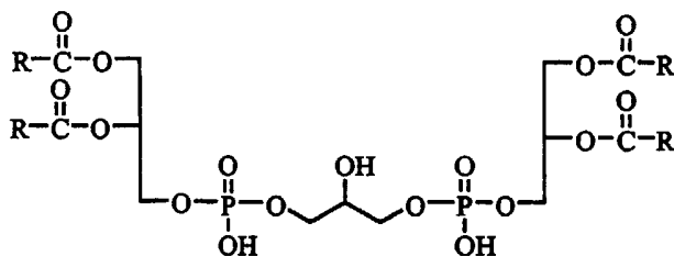
Cardiolipin
