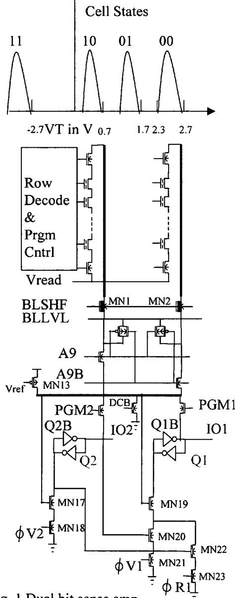
Fig. 1 Dual bit sense amp
