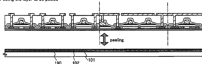
(B) Peeling the layer to be peeled
