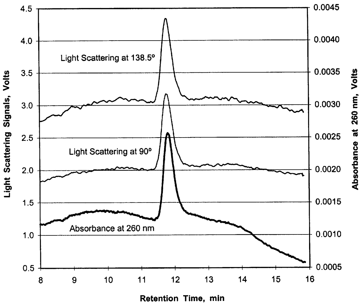
Comparison of Sensitivities of Viral Detection by Light Scattering and Absorbance, with a 1000:1 Ratio of Voltage Scales
