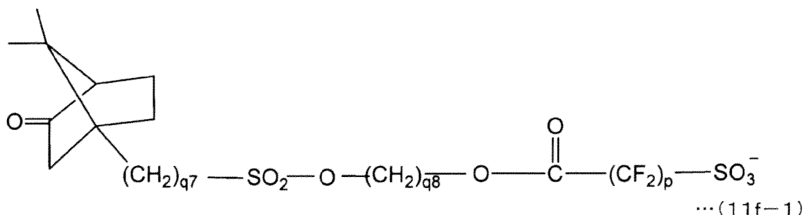
[Chemical Formula 16]
