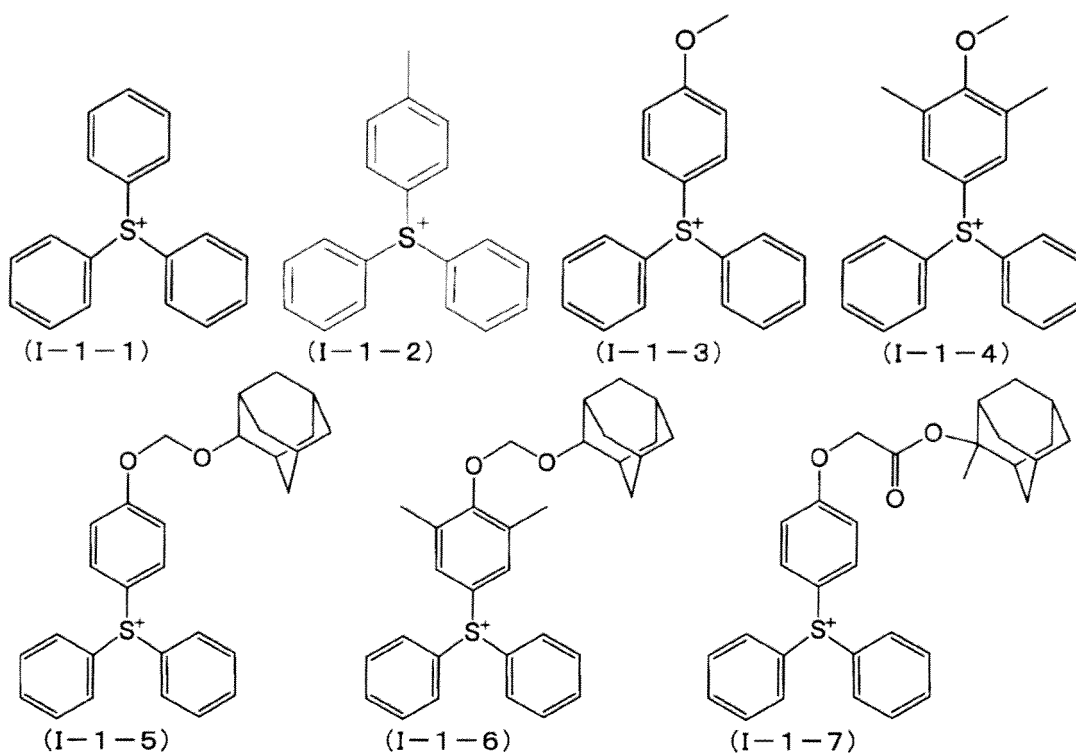
[Chemical Formula 62]
