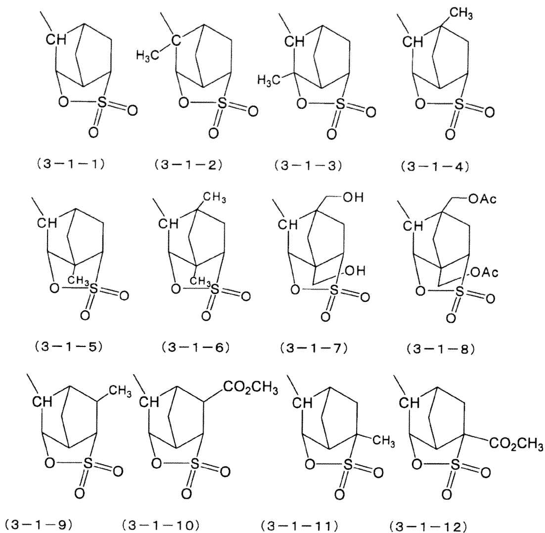
[Chemical Formula 41]
