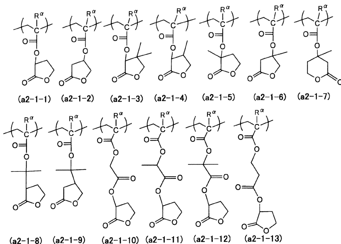
[Chemical Formula 51]
