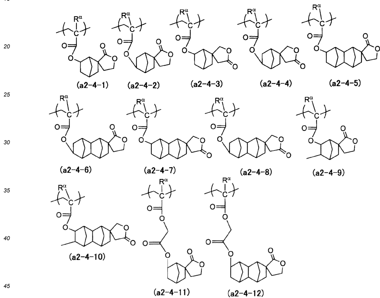
[Chemical Formula 53]
