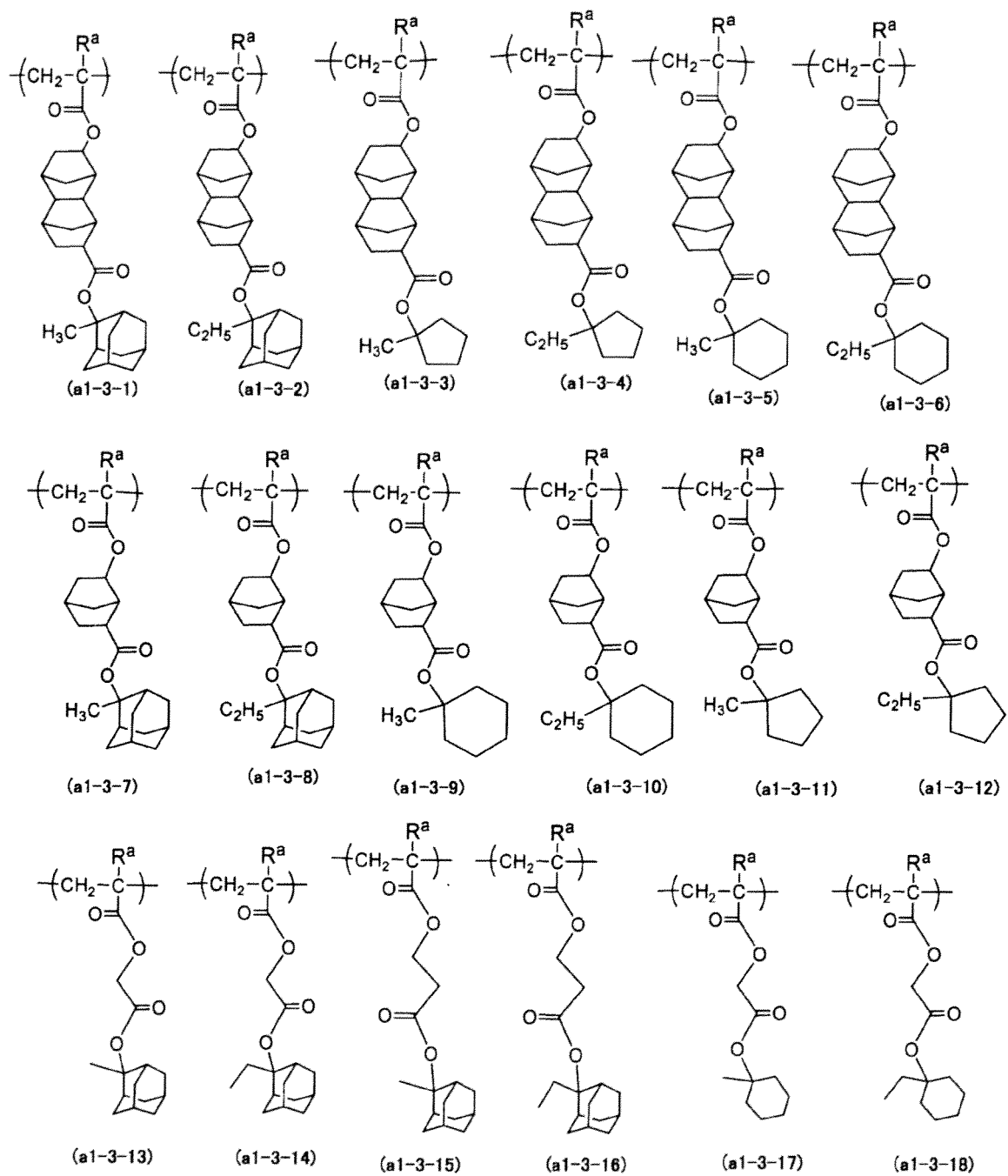
[Chemical Formula 33]
