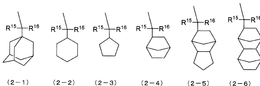
[Chemical Formula 23]
