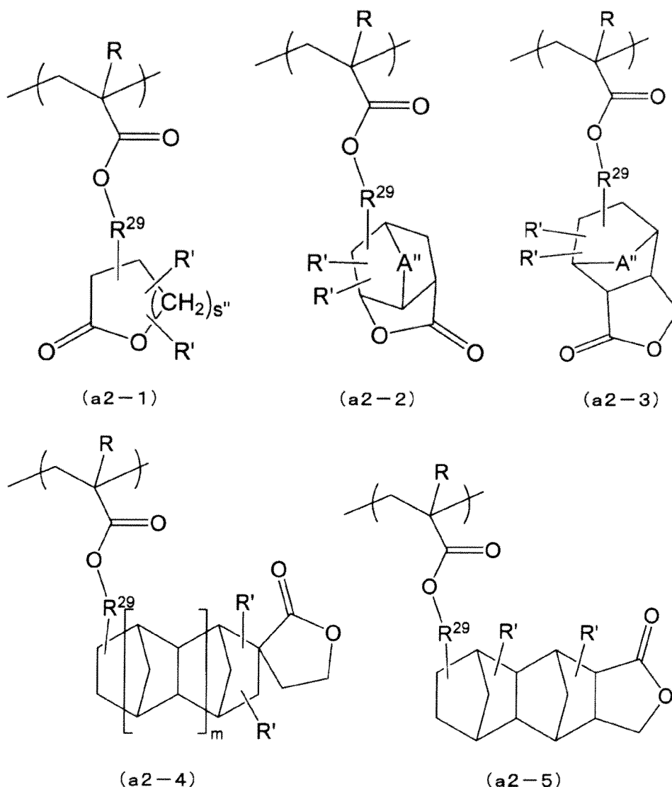
[Chemical Formula 49]
