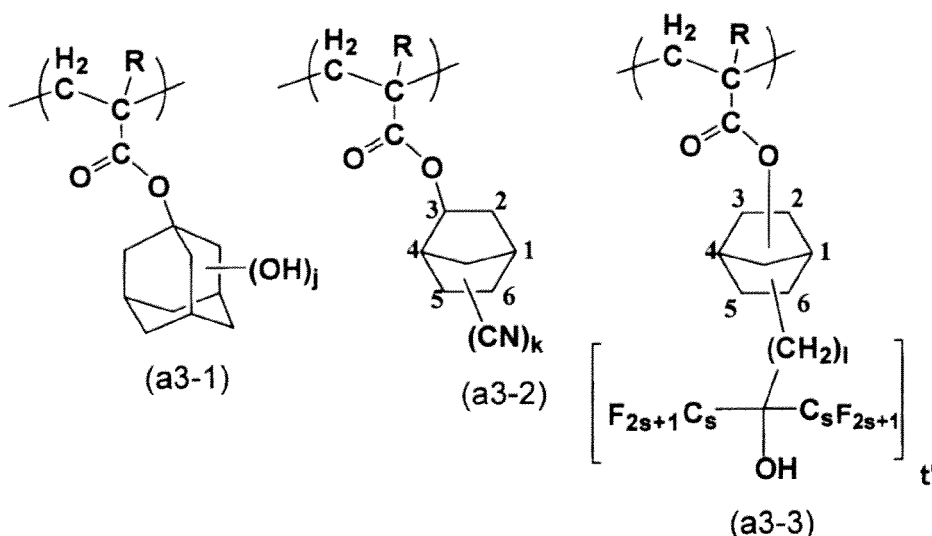
[Chemical Formula 55]
