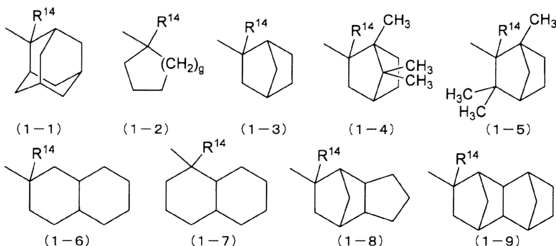
[Chemical Formula 22]
