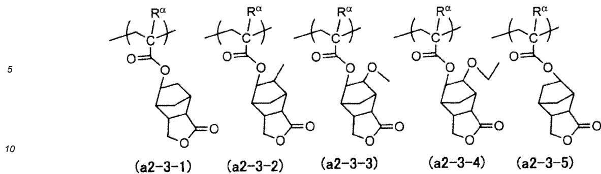
[Chemical Formula 53]
