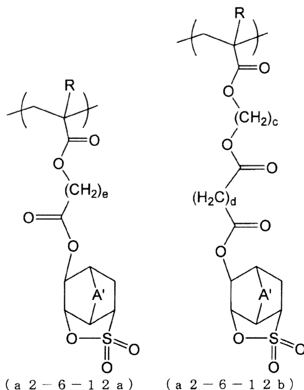
[Chemical Formula 48]
