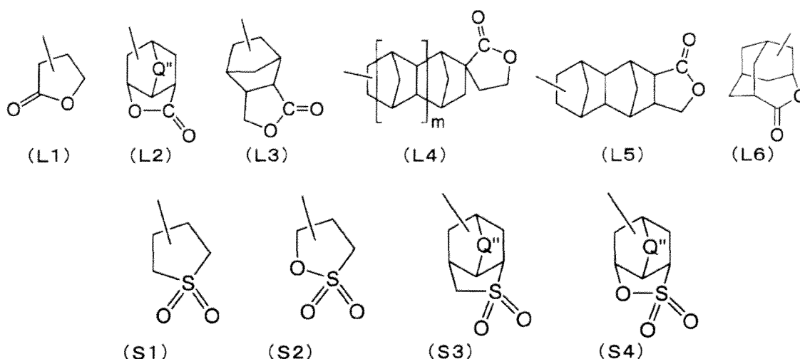
[Chemical Formula 7]
