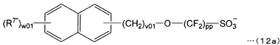
[Chemical Formula 17]
