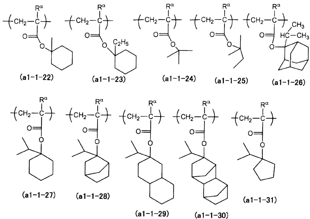
[Chemical Formula 31]
