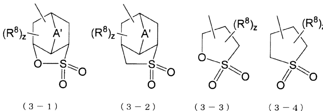
[Chemical Formula 39]
