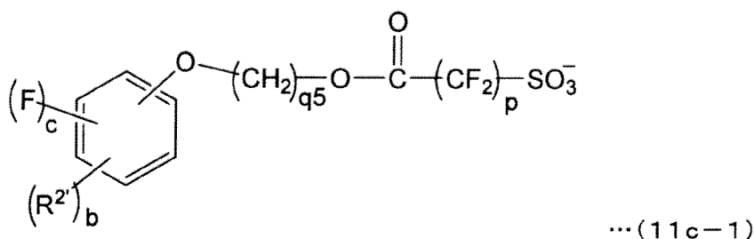
[Chemical Formula 12]
