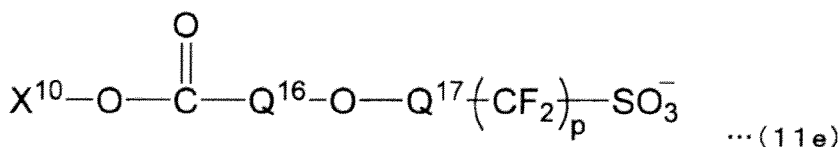
[Chemical Formula 14]
