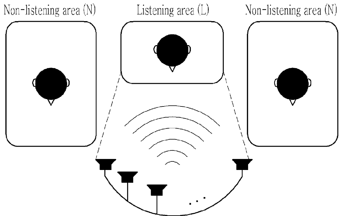
One-dimensional straight array type of sound source
