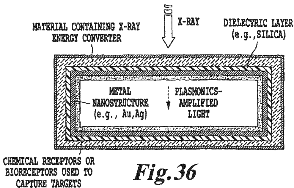
STERILIZATION SYSTEM 10 WITH PLASMONICS AND CHEMICAL RECEPTORS OR BIORECEPTORS
