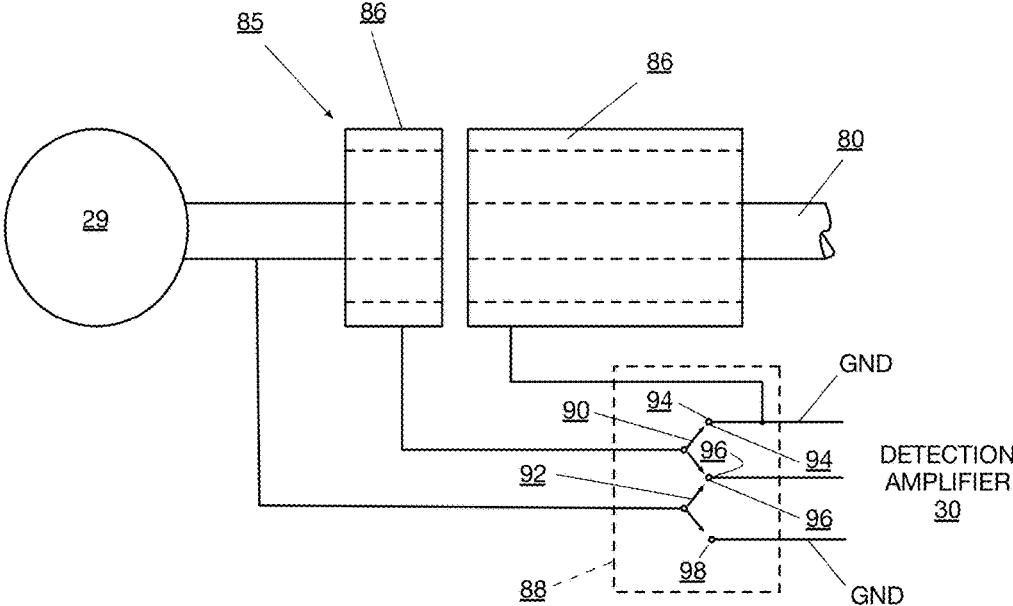
Fig. 42 (PRIOR ART)
