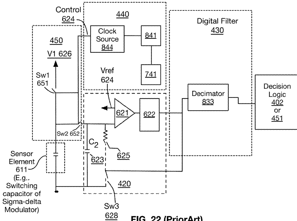
FIG. 22 (Prior Art)
