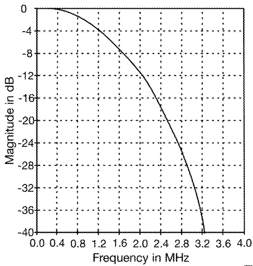
Inphase Filter Frequency Response
