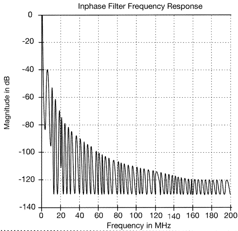
Inphase Filter Frequency Response
