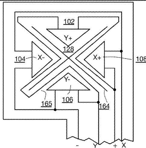
Fig. 40 (Prior Art)
