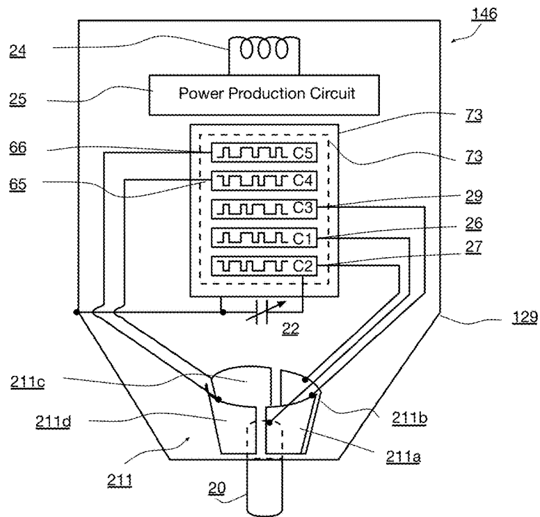
Fig.43 (Prior Art)
