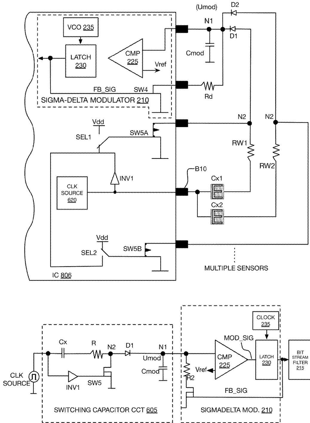
FIG. 20 (Prior Art)
