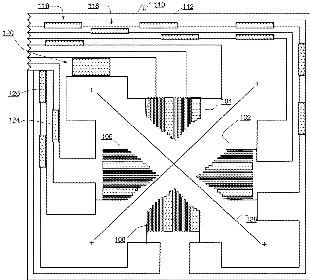
Fig. 40 (Prior Art)
