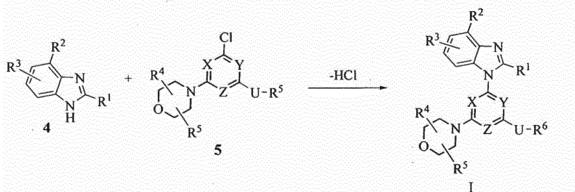
Scheme 4
