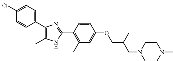
1-(3-{4-[4-(4-Chloro-phenyl)-5-methyl-1H-imidazol-2-yl]-3-methyl-phenoxy}-2-methyl-propyl)-4-methyl-piperazine
