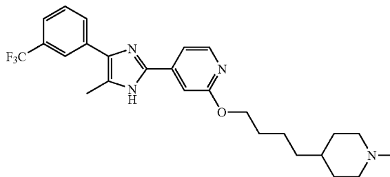
2-[4-(1-Methyl-piperidin-4-yl)-butoxy]-4-[5-methyl-4-(3-trifluoromethyl-phenyl)-1H-imidazol-2-yl]-pyridine
