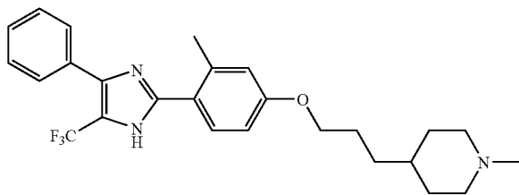
1-Methyl-4-{3-[3-methyl-4-(4-phenyl-5-trifluoromethyl-1H-imidazol-2-yl)-phenoxy]-propyl}-piperidine
