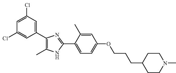
4-(3-(4-[4-(3,5-Dichloro-phenyl)-5-methyl-1H-imidazol-2-yl]-3-methyl-phenoxy}-propyl)-1-methyl-piperidine
