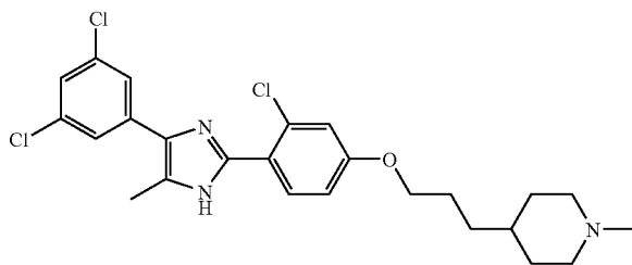
4-(3-(3-Chloro-4-[4-(3,5-dichloro-phenyl)-5-methyl-1H-imidazol-2-yl]-phenoxy}-propyl)-1-methyl-piperidine
