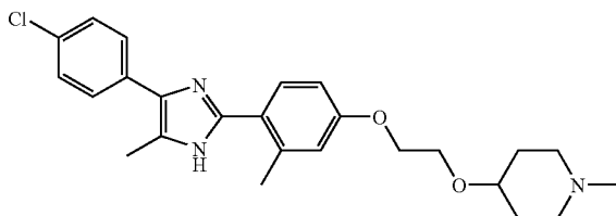
4-(2-{4-[4-(4-Chloro-phenyl)-5-methyl-1H-imidazol-2-yl]-3-methyl-phenoxy}-ethoxy)-1-methyl-piperidine
