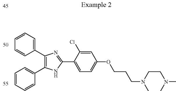
1-{3-[3-Chloro-4-(4,5-diphenyl-1H-imidazol-2-yl)-phenoxy]-propyl}-4-methyl-piperazine
