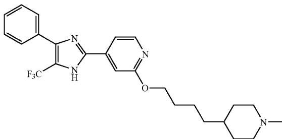
2-[4-(1-Methyl-piperidin-4-yl)-butoxy]-4-[5-methyl-4-(3-trifluoromethyl-phenyl)-1H-imidazol-2-yl]-pyridine
