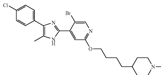
5-Bromo-4-[4-(4-chloro-phenyl)-5-methyl-1H-imidazol-2-yl]-2-[4-(1-methyl-piperidin-4-yl)-butoxy]-pyridine
