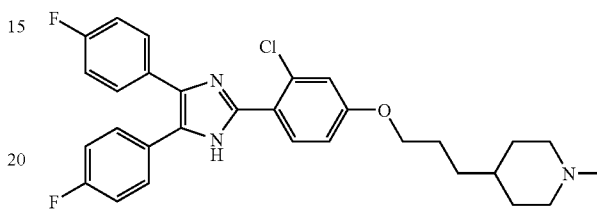
4-(3-(4-[4,5-Bis-(4-fluoro-phenyl)-1H-imidazol-2-yl]-3-chloro-phenoxy}-propyl)-1-methyl-piperidine
