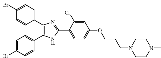
1-(3-{4-[4,5-Bis-(4-bromo-phenyl)-1H-imidazol-2-yl]-3-chloro-phenoxy}-propyl)-4-methyl-piperazine
