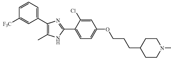
4-(3-{3-Chloro-4-[5-methyl-4-(3-trifluoromethyl-phenyl)-1H-imidazol-2-yl]-phenoxy}-propyl)-1-methyl-piperidine
