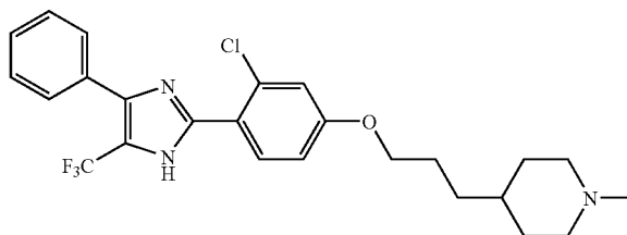
4-{3-[3-Chloro-4-(4-phenyl-5-trifluoromethyl-1H-imidazol-2-yl)-phenoxy]-propyl}-1-methyl-piperidine
