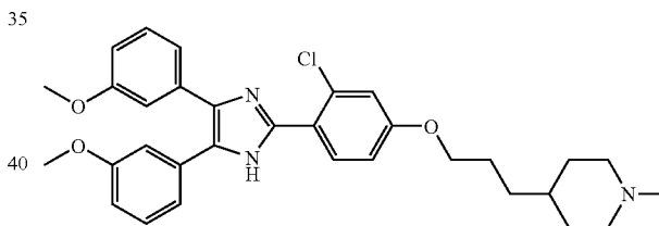
4-(3-(4-[4,5-Bis-(3-methoxy-phenyl)-1H-imidazol-2-yl]-3-chloro-phenoxy}-propyl)-1-methyl-piperidine
