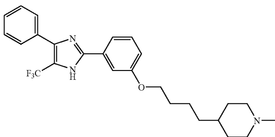
1-Methyl-4-[4-[3-(4-phenyl-5-trifluoromethyl-1H-imidazol-2-yl)-phenoxy]-butyl]-piperidine
