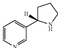
(S)-Nornicotine (5)
