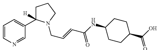
(1R,4s)-4-((E)-4-((S)-2-(pyridin-3-yl)pyrrolidin-1-yl)but-2-enamido)cyclohexanecarboxylic acid (29)
