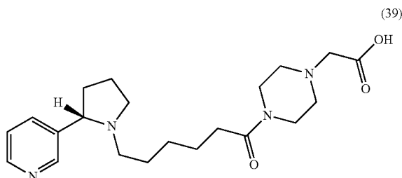
(S)-2-(4-(6-(2-(Pyridin-3-yl)pyrrolidin-1-yl)hexanoyl)piperazin-1-yl)acetic acid (39)
