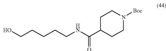
tert-Butyl 4-((5-hydroxypentyl)carbamoyl)piperidine-1-carboxylate (44)
