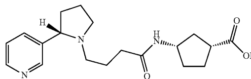
(1R,3S)-3-(4-((S)-2-(pyridin-3-yl)pyrrolidin-1-yl)butanamido)cyclopentanecarboxylic acid (33)
