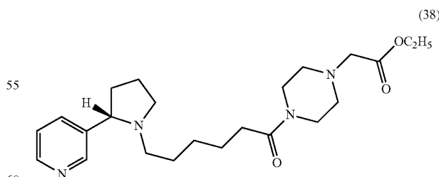
(S)-Ethyl 2-(4-(6-(2-(pyridin-3-yl)pyrrolidin-1-yl)hexanoyl)piperazin-1-yl)acetate (38)
