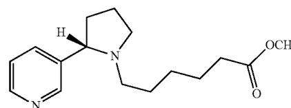
(S)-Methyl 6-(2-(pyridin-3-yl)pyrrolidin-1-yl)hexanoate (6b)
