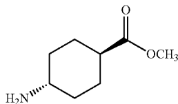
(1r,4r)-Methyl 4-aminocyclohexanecarboxylate (12)
