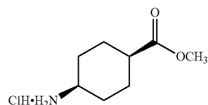
(1s,4s)-Methyl 4-aminocyclohexanecarboxylate hydrochloride (14)
