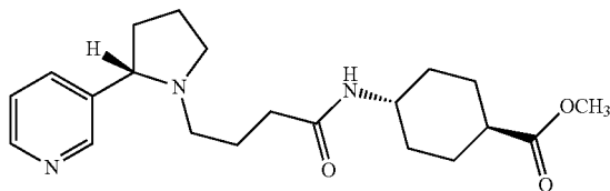
(1S,4R)-Methyl 4-(4-((S)-2-(pyridin-3-yl)pyrrolidin-1-yl)butanamido)cyclohexanecarboxylate (22)
