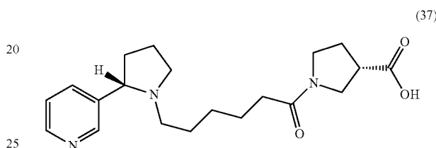
(S)-1-(6-((S)-2-(Pyridin-3-yl)pyrrolidin-1-yl)hexanoyl)pyrrolidine-3-carboxylic acid (37)
