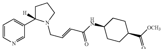
(1R,4s)-Methyl 4-((E)-4-((S)-2-(pyridin-3-yl)pyrrolidin-1-yl)but-2-enamido)cyclohexane-carboxylate (28)
