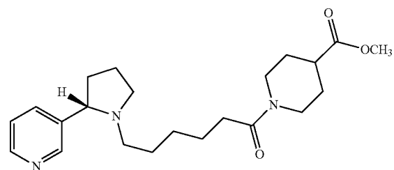
(S)-Methyl 1-(6-(2-(pyridin-3-yl)pyrrolidin-1-yl)hexanoyl)piperidine-4-carboxylate (34)
