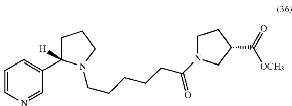
(S)-Methyl 1-(6-((S)-2-(pyridin-3-yl)pyrrolidin-1-yl)hexanoyl)pyrrolidine-3-carboxylate (36)
