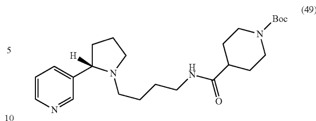
(S)-tert-Butyl 4-((4-(2-(pyridin-3-yl)pyrrolidin-1-yl)butyl)carbamoyl)piperidine-1-carboxylate (49)
