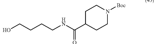
tert-Butyl 4-((4-hydroxybutyl)carbamoyl)piperidine-1-carboxylate (43)
