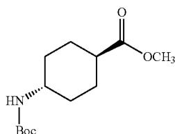
(1r,4r)-Methyl 4-((tert-butoxycarbonyl)amino)cyclohexanecarboxylate (11)
