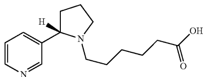
(S)-6-(2-(Pyridin-3-yl)pyrrolidin-1-yl)hexanoic acid (7b)
