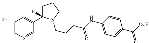
(S)-Methyl 4-(4-(2-(pyridin-3-yl)pyrrolidin-1-yl)butanamido)benzoate (30)
