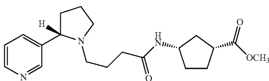
(1R,3S)-Methyl 3-(4-((S)-2-(pyridin-3-yl)pyrrolidin-1-yl)butanamido)cyclopentane-carboxylate (32)
