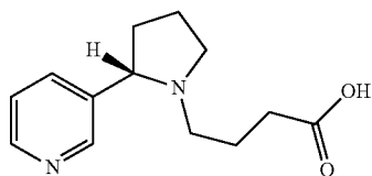
(S)-4-(2-(Pyridin-3-yl)pyrrolidin-1-yl)butanoic acid (7a)
