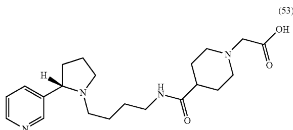
(S)-2-(4-((4-(2-(pyridin-3-yl)pyrrolidin-1-yl)butyl)carbamoyl)piperidin-1-yl)acetic acid (53)
