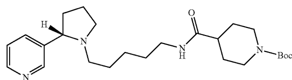
(S)-tert-Butyl 4-((5-(2-(pyridin-3-yl)pyrrolidin-1-yl)pentyl)carbamoyl)piperidine-1-carboxylate (50)
