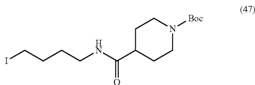
tert-Butyl 4-((4-iodobutyl)carbamoyl)piperidine-1-carboxylate (47)
