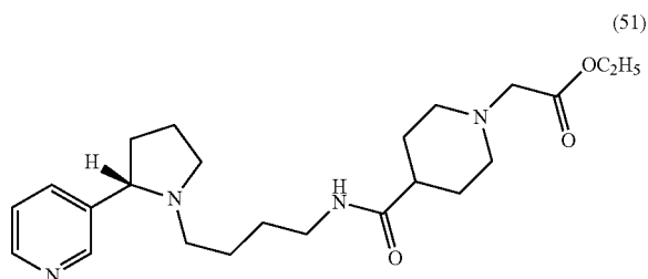
(S)-Ethyl 2-(4-((4-(2-(pyridin-3-yl)pyrrolidin-1-yl)butyl)carbamoyl)piperidin-1-yl)acetate (51)
