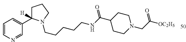
(S)-Ethyl 2-(4-((5-(2-(pyridin-3-yl)pyrrolidin-1-yl)pentyl)carbamoyl)piperidin-1-yl)acetate (52)
