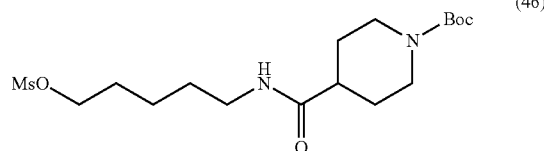
tert-Butyl 4-((5-((methylsulfonyl)oxy)pentyl)carbamoyl)piperidine-1-carboxylate (46)
