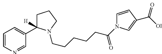
(S)-1-(6-(2-(Pyridin-3-yl)pyrrolidin-1-yl)hexanoyl)-1H-pyrrole-3-carboxylic acid (41)
