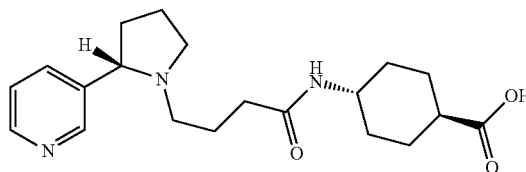
(1S,4R)-4-(4-((S)-2-(pyridin-3-yl)pyrrolidin-1-yl)butanamido)cyclohexanecarboxylic acid (23)
