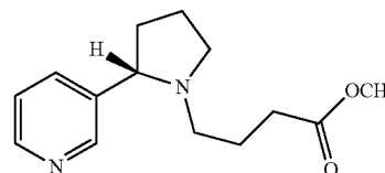
(S)-Methyl 4-(2-(pyridin-3-yl)pyrrolidin-1-yl)butanoate (6a)
