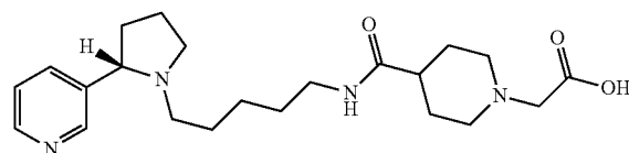
(S)-2-(4-((5-(2-(pyridin-3-yl)pyrrolidin-1-yl)pentyl)carbamoyl)piperidin-1-yl)acetic acid (54)
