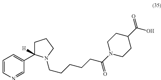
(S)-1-(6-(2-(Pyridin-3-yl)pyrrolidin-1-yl)hexanoyl)piperidine-4-carboxylic acid (35)
