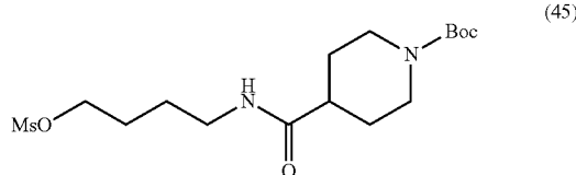
tert-Butyl 4-((4-((methylsulfonyl)oxy)butyl)carbamoyl)piperidine-1-carboxylate (45)
