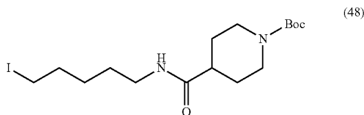
tert-Butyl 4-((5-iodopentyl)carbamoyl)piperidine-1-carboxylate (48)
