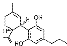
Cannabidivarin (CBDV)
