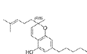
(±)-Cannabichromene CBC-C 5
