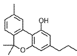
Cannabivarin (CBV)
