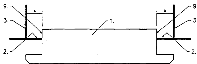
SECTION F-F
