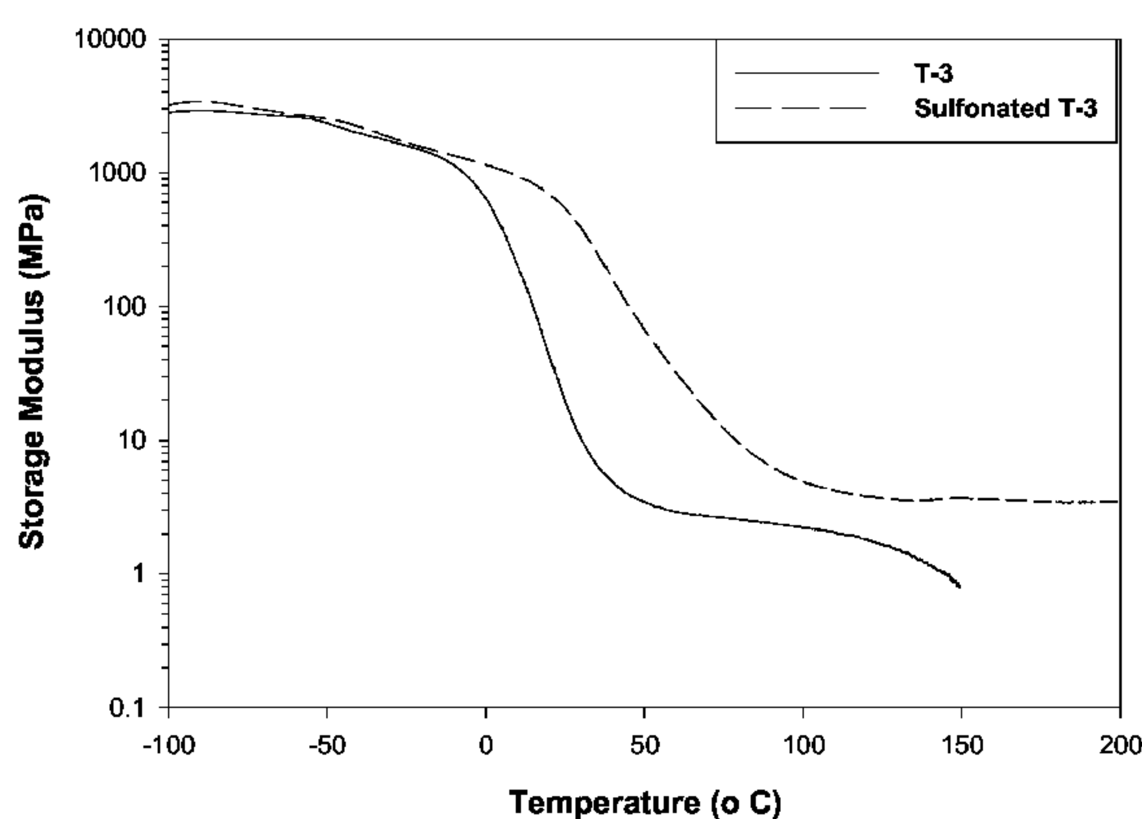
Polymer T-3 Before and After Sulfonation
