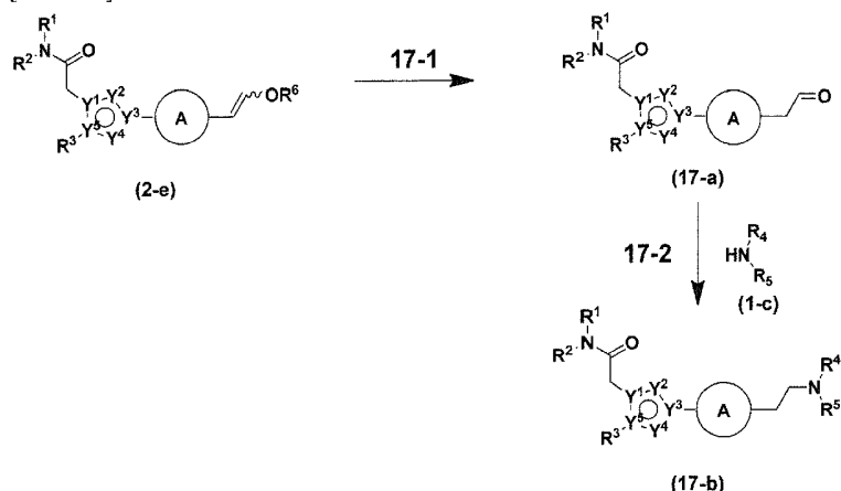
Scheme 17
