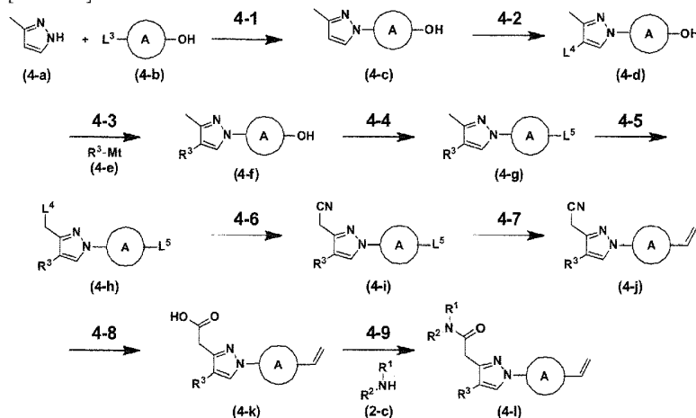
Scheme 4
