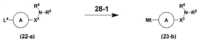
Scheme 28
