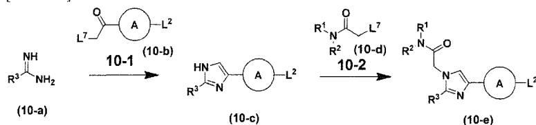
Scheme 10
