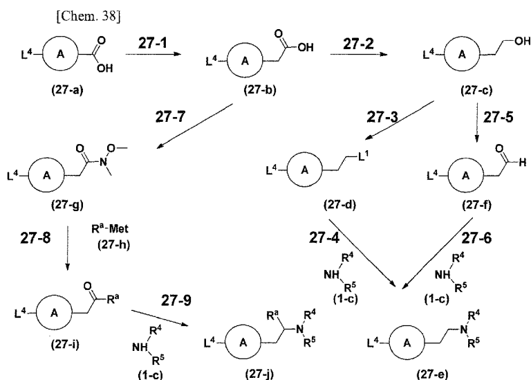
Scheme 27
