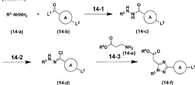
Scheme 14
