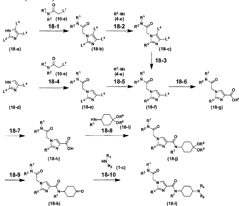
Scheme 18
