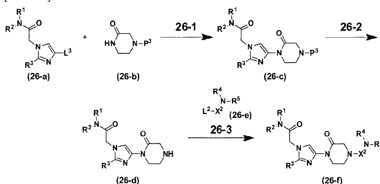
Scheme 26
