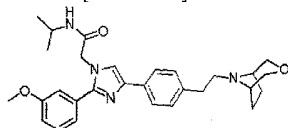
[Chem. 267]
