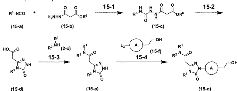
Scheme 15
