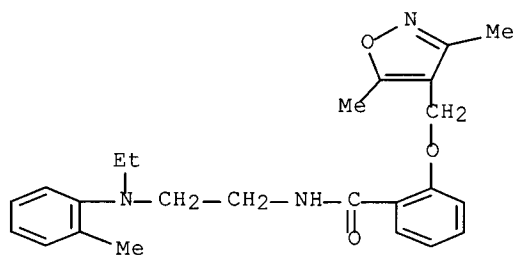
2-[(3,5-dimethyl-4-isoxazolyl)methoxy]-N-[2-[ethyl(3-methylphenyl)amino]ethyl]-
