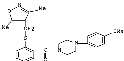
[4-(2,6-dimethyl-4-pyrimidinyl)-1-piperazinyl][2-[(2-thienylmethyl)thio]phenyl]-methanone
