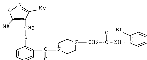
N-phenyl-4-[2-[(2-thienylmethyl)thio]benzoyl]-1-piperazineacetamide
