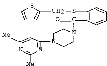
[4-(2,6-dimethyl-4-pyrimidinyl)-1-piperazinyl][2-[(2-thienylmethyl)thio]phenyl]-methanone
