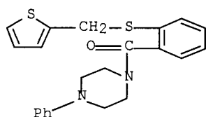
(4-phenyl-1-piperazinyl)[2-[(2-thienylmethyl)thio]phenyl]-methanone
