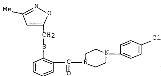
[2-[[[(3-methyl-1,2,4-oxadiazol-5-yl)methyl]thio]phenyl][4-(3-methylphenyl)-1-piperazinyl]-methanone
