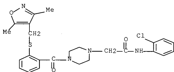
4-[2-[[[(3,5-dimethyl-4-isoxazolyl)methyl]thio]benzoyl]-N-phenyl-1-piperazineacetamide
