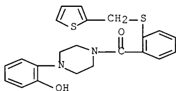
2-[(3-thienylmethyl)thio]phenyl[4-[5-(trifluoromethyl)-2-pyridinyl]-1-piperazinyl]-methanone
