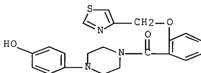
[4-(4-hydroxyphenyl)-1-piperazinyl][2-(4-thiazolylmethoxy)phenyl]-methanone
