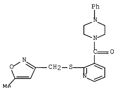
[2-[[[(5-methyl-3-isoxazolyl)methyl]thio]-3-pyridinyl](4-phenyl-1-piperazinyl)-methanone
