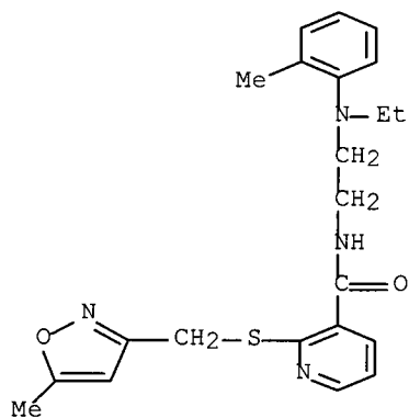
N-[2-[ethyl(2-methylphenyl)amino]ethyl]-2-[[[(5-methyl-3-isoxazolyl)methyl]thio]-3-pyridinecarboxamide
