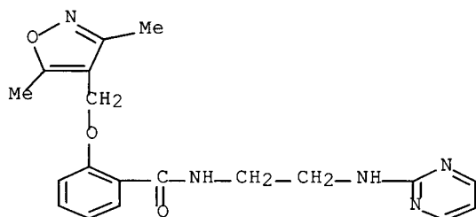
2-[(3,5-dimethyl-4-isoxazolyl)methoxy]-N-[1-methyl-2-(methylphenylamino)ethyl]-benzamide
