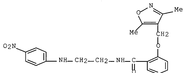
2-[(3,5-dimethyl-4-isoxazolyl)methoxy]-N-[2-[ethyl(2-methylphenyl)amino]ethyl]-
