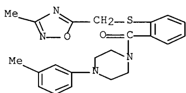
[2-[[[(3-methyl-1,2,4-oxadiazol-5-yl)methyl]thio]phenyl][4-(3-methylphenyl)-1-piperazinyl]-methanone
