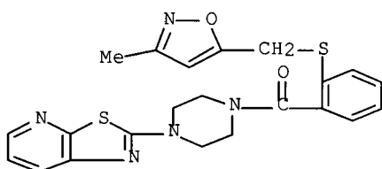
[2-[[[(3-methyl-5-isoxazolyl)methyl]thio]phenyl](4-thiazolo[5,4-b]pyridin-2-yl-1-piperazinyl)-methanone
