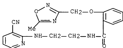
2-[(3,5-dimethyl-4-isoxazolyl)methoxy]-N-[2-[(4-nitrophenyl)amino]ethyl]- benzamide
