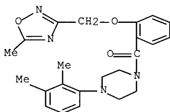
[4-(2,3-dimethylphenyl)-1-piperazinyl][2-[(5-methyl-1,2,4-oxadiazol-3-yl)methoxy]phenyl]-methanone
