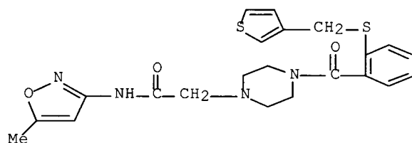
4-[[2-[[[(3,5-dimethyl-4-isoxazolyl)methyl]thio]-3-pyridinyl]carbonyl]-N-(5-methyl-3-isoxazolyl)- 1-piperazineacetamide
