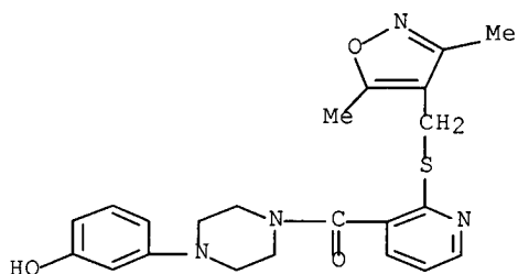
[2-[[[(3,5-dimethyl-4-isoxazolyl)methyl]thio]phenyl][4-(1-methyl-1H-imidazol-2-yl)-1-piperazinyl]-methanone
