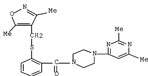
[2-[[[(3,5-dimethyl-4-isoxazolyl)methyl]thio]phenyl][4-(2,6-dimethyl-4-pyrimidinyl)-1-piperazinyl]-methanone
