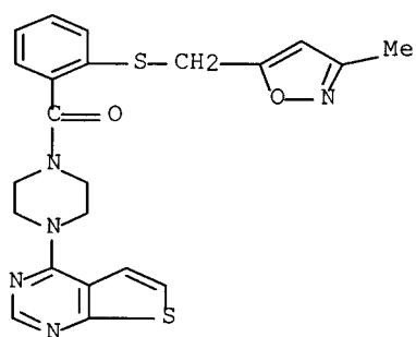
[2-[[[(3-methyl-5-isoxazolyl)methyl]thio]phenyl][4-(2-pyridinyl)-1-piperazinyl]-methanone
