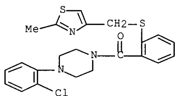
[4-(2-chlorophenyl)-1-piperazinyl][2-[[2-methyl-4-thiazolyl)methyl]thio]phenyl]-methanone
