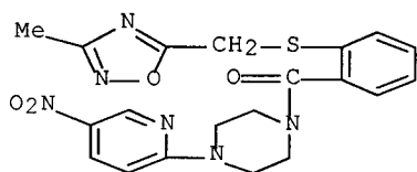
[2-[[5-methyl-1,2,4-oxadiazol-3-yl)methyl]thio]phenyl][4-[5-(trifluoromethyl)-2-pyridinyl]-1-piperazinyl]-methanone
