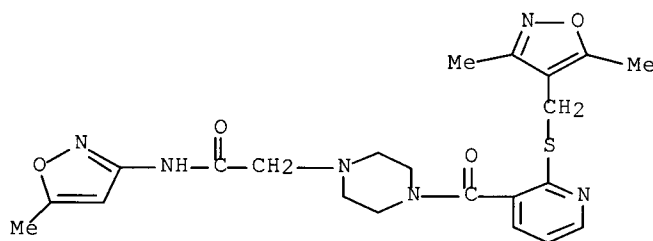
4-[[2-[[[(3,5-dimethyl-4-isoxazolyl)methyl]thio]-3-pyridinyl]carbonyl]-N-(5-methyl-3-isoxazolyl)- 1-piperazineacetamide
