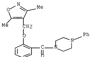
[2-[(3,5-dimethyl-4-isoxazolyl)methoxy]phenyl](4-phenyl-1-piperazinyl)-methanone
