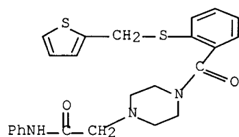
N-(2-chlorophenyl)-4-[2-[[[(3,5-dimethyl-4-isoxazolyl)methyl]thio]benzoyl]-1-piperazineacetamide
