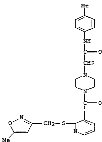
N-(5-methyl-3-isoxazolyl)-4-[2-[(2-thienylmethyl)thio]benzoyl]- 1-piperazineacetamide
