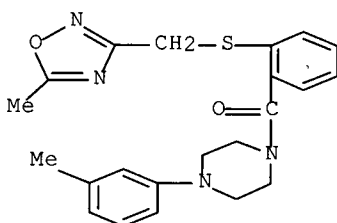
6-[4-[2-[[[(5-methyl-1,2,4-oxadiazol-3-yl)methyl]thio]benzoyl]-1-piperazinyl]-3-Pyridinecarbonitrile
