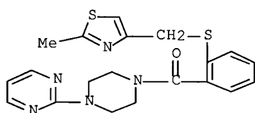
[2-[[[(2-methyl-4-thiazolyl)methyl]thio]phenyl][4-(2-pyrimidinyl)-1-piperazinyl]-methanone
