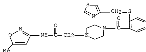
N-(2-ethylphenyl)-4-[2-[(3-thienylmethyl)thio]benzoyl]- 1-piperazineacetamide
