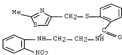
2-[[[(2-methyl-4-thiazolyl)methyl]thio]-N-[2-[(2-nitrophenyl)amino]ethyl]- benzamide
