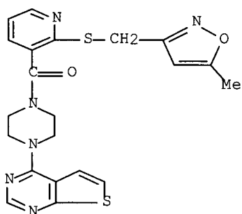
[2-[[[(5-methyl-3-isoxazolyl)methyl]thio]-3-pyridinyl](4-thieno[2,3-d]pyrimidin-4-yl)-1-piperazinyl]-methanone
