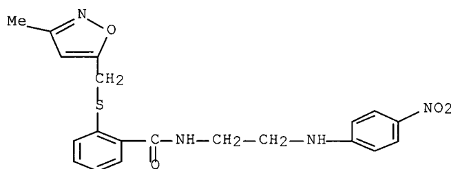
2-[[[(3-methyl-5-isoxazolyl)methyl]thio]-N-[2-[(4-nitrophenyl)amino]ethyl]- benzamide
