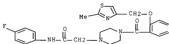
5 N-(4-fluorophenyl)-4-[2-[(2-methyl-4-thiazolyl)methoxy]benzoyl]- 1-piperazineacetamide
