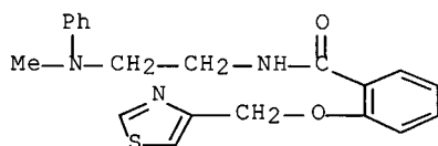
N-[2-(methylphenylamino)propyl]-2-(4-thiazolylmethoxy)- benzamide
