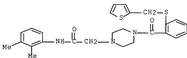
10 4-[2-[[[(3,5-dimethyl-4-isoxazolyl)methyl]thio]benzoyl]-N-(2-ethylphenyl)-1-piperazineacetamide
