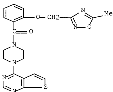
5 [2-[(3,5-dimethyl-4-isoxazolyl)methoxy]phenyl][4-(4-fluorophenyl)-1-piperazinyl]-methanone
