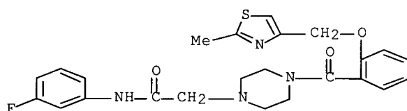
N-(2,6-dimethylphenyl)-4-[2-[(5-methyl-1,2,4-oxadiazol-3-yl)methoxy]benzoyl]- 1-piperazineacetamide
