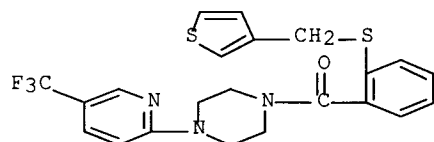
2-[(3-thienylmethyl)thio]phenyl[4-[5-(trifluoromethyl)-2-pyridinyl]-1-piperazinyl]-methanone
