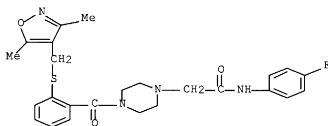
5 N-(2,3-dimethylphenyl)-4-[[2-[[[(5-methyl-3-isoxazolyl)methyl]thio]-3-pyridinyl]carbonyl]-1-piperazineacetamide
