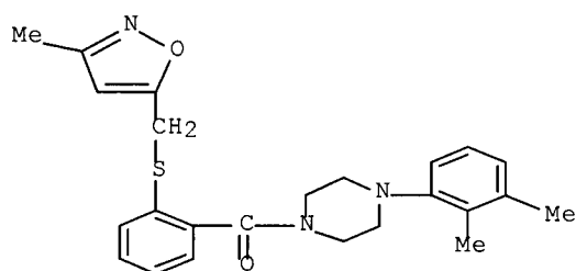
[4-(2,3-dimethylphenyl)-1-piperazinyl][2-[(3-methyl-5-isoxazolyl)methyl]thio]phenyl-methanone
