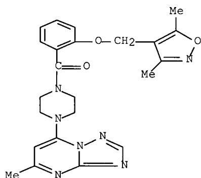
[2-[(3,5-dimethyl-4-isoxazolyl)methoxy]phenyl][4-(5-methyl[1,2,4]triazolo[1,5-a]pyrimidin-7-yl)-1-piperazinyl]-methanone
