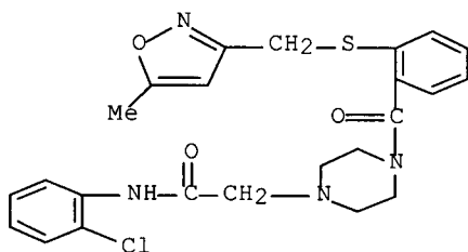
N-(2,3-dimethylphenyl)-4-[2-[(2-thienylmethyl)thio]benzoyl]- 1-piperazineacetamide
