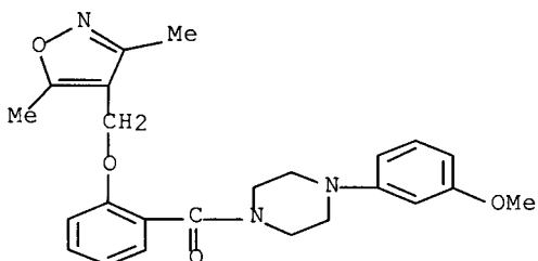
[4-(3-methylphenyl)-1-piperazinyl][2-(4-thiazolylmethoxy)phenyl]-methanone
