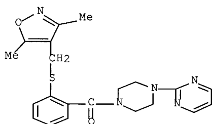
5 [2-[[[(3,5-dimethyl-4-isoxazolyl)methyl]thio]-3-pyridinyl][4-(thieno[2,3-d]pyrimidin-4-yl)-1-piperazinyl]-methanone
