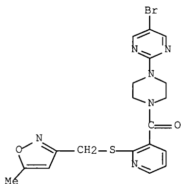
[2-[[[(3,5-dimethyl-4-isoxazolyl)methyl]thio]phenyl][4-(2-pyrimidinyl)-1-piperazinyl]-methanone
