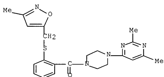
[4-(2,6-dimethyl-4-pyrimidinyl)-1-piperazinyl][2-[(3-methyl-5-isoxazolyl)methyl]thio]phenyl]-methanone
