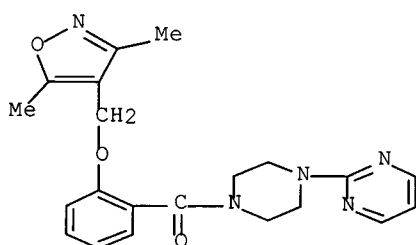
[2-[(3,5-dimethyl-4-isoxazolyl)methoxy]phenyl][4-(2-pyrimidinyl)-1-piperazinyl]-methanone
