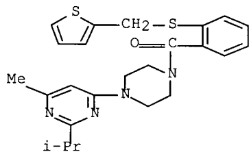
[4-[6-methyl-2-(1-methylethyl)-4-pyrimidinyl]-1-piperazinyl][2-[(2-thienylmethyl)thio]phenyl]-methanone
