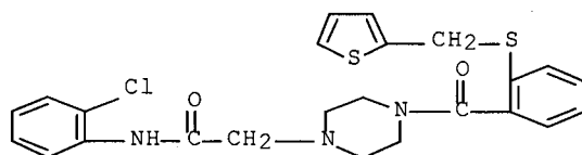
N-phenyl-4-[2-[(3-thienylmethyl)thio]benzoyl]-1-piperazineacetamide
