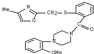
[2-[(3,5-dimethyl-4-isoxazolyl)methoxy]phenyl][4-(2,3-dimethylphenyl)-1-piperazinyl]-methanone
