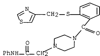
N-phenyl-4-[2-[(4-thiazolylmethyl)thio]benzoyl]-1-piperazineacetamide
