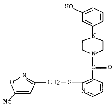
[2-[[[(3,5-dimethyl-4-isoxazolyl)methyl]thio]-3-pyridinyl](4-thiazolo[5,4-b]pyridin-2-yl-1-piperazinyl)-methanone
