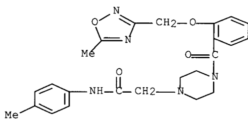
N-(2-ethylphenyl)-4-[2-[(5-methyl-1,2,4-oxadiazol-3-yl)methoxy]benzoyl]- 1-piperazineacetamide
