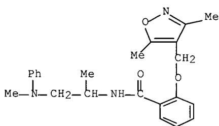
2-[(3,5-dimethyl-4-isoxazolyl)methoxy]-N-[1-methyl-2-(methylphenylamino)ethyl]-benzamide
