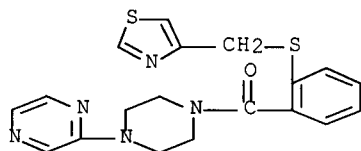
2-[4-[2-[(4-thiazolylmethyl)thio]benzoyl]-1-piperazinyl]-4-Pyridinecarbonitrile,
