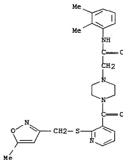
N-(4-fluorophenyl)-4-[2-[(3-thienylmethyl)thio]benzoyl]- 1-piperazineacetamide
