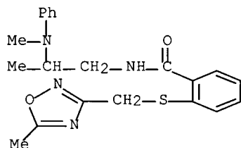
2-[[[(3-methyl-5-isoxazolyl)methyl]thio]-N-[2-[(4-nitrophenyl)amino]ethyl]- benzamide
