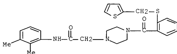
N-(2,3-dimethylphenyl)-4-[2-[(2-thienylmethyl)thio]benzoyl]-1-piperazineacetamide
