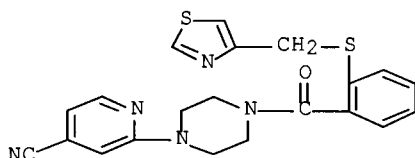
[2-[[[(3,5-dimethyl-4-isoxazolyl)methyl]thio]phenyl][4-(2-ethoxyphenyl)-1-piperazinyl]-methanone
