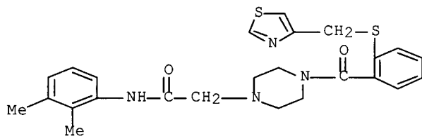
N-(2,3-dimethylphenyl)-4-[2-[(2-thienylmethyl)thio]benzoyl]-1-piperazineacetamide
