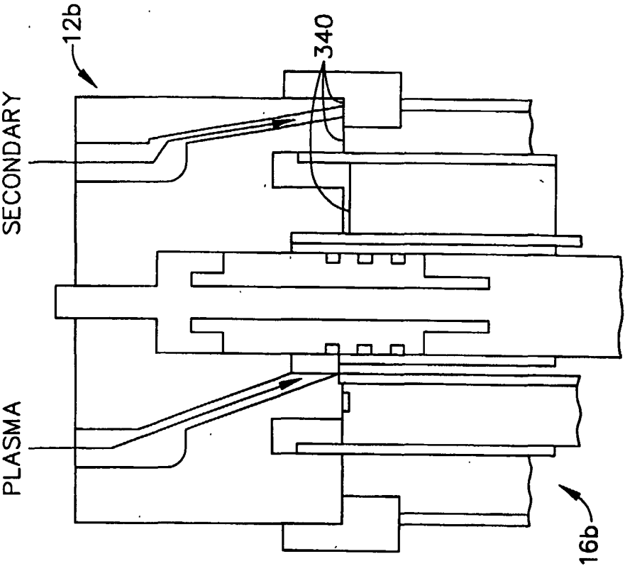
FIG. 32b (GAS PASSAGEWAYS)
