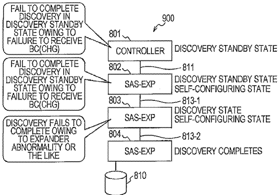
FIG. 33 RELATED ART
