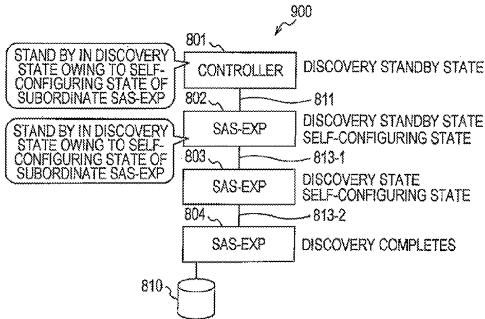
FIG. 32 RELATED ART
