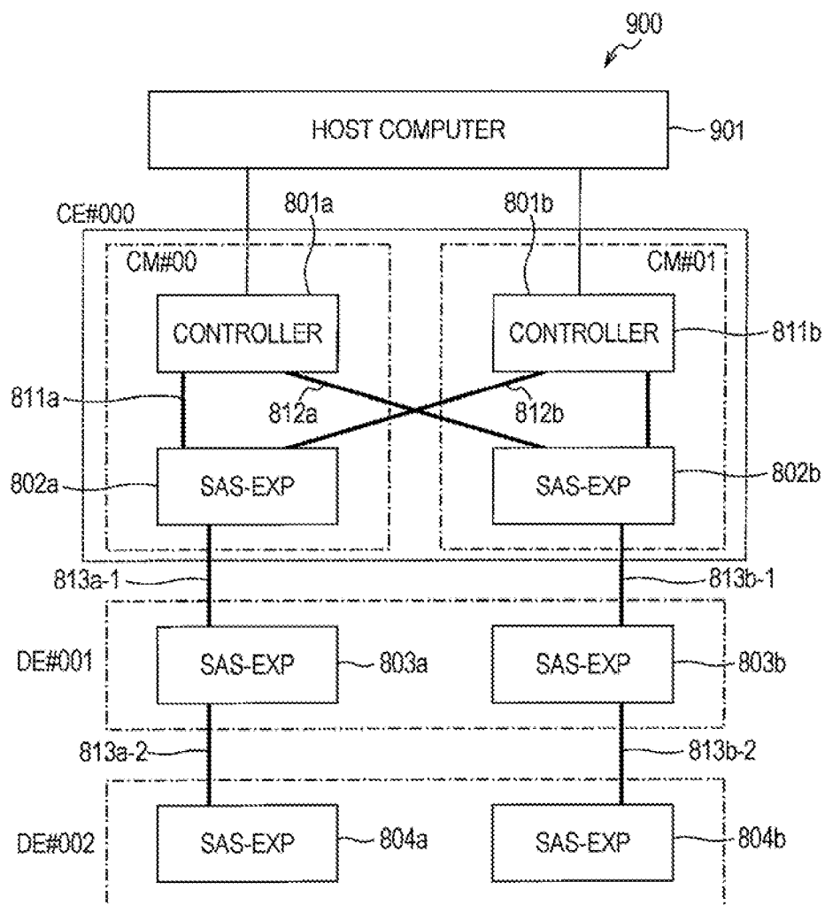
FIG. 29 RELATED ART
