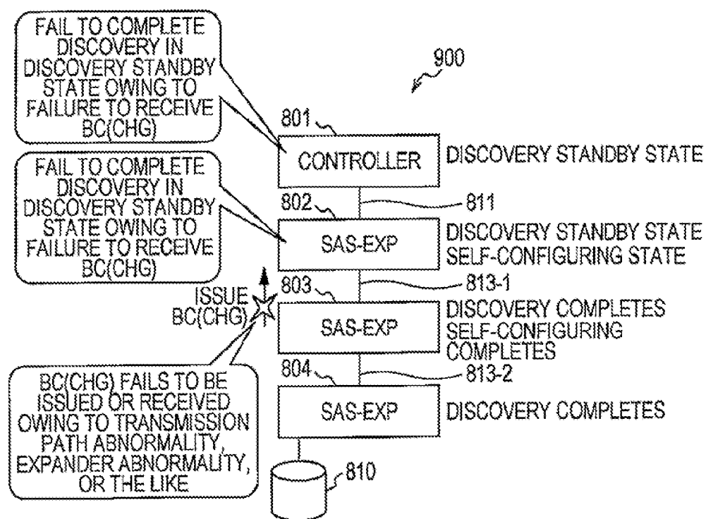
FIG. 34 RELATED ART
