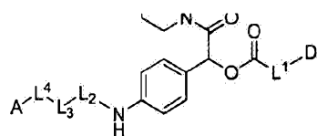
(Compound Z)
