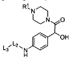
(Compound X 1 )
