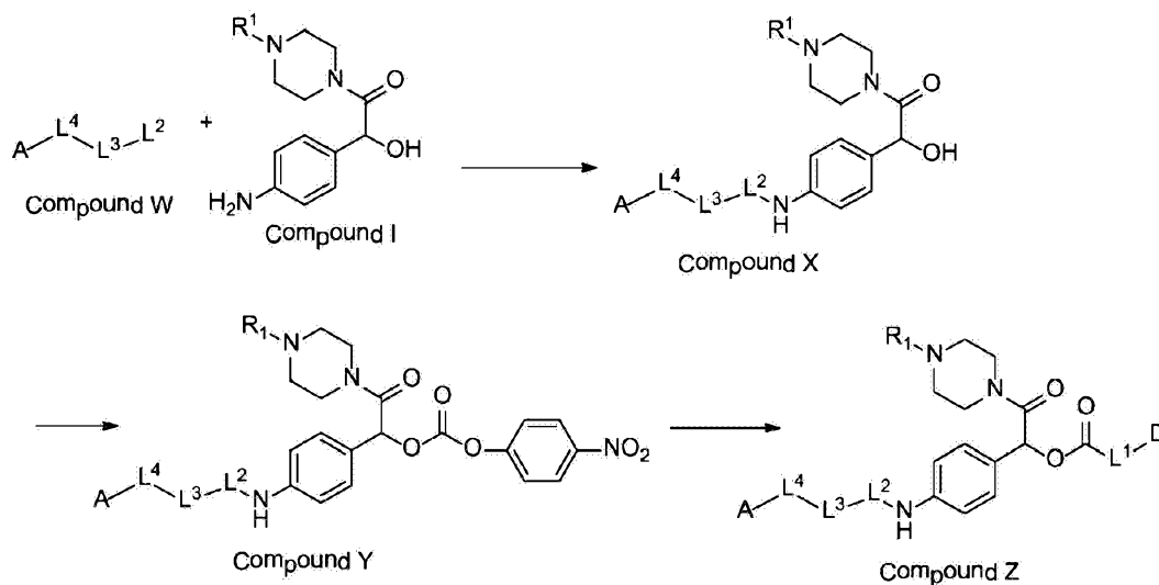
Scheme 4
