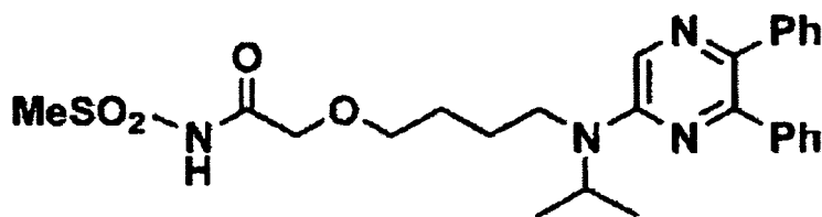
Compound 2
