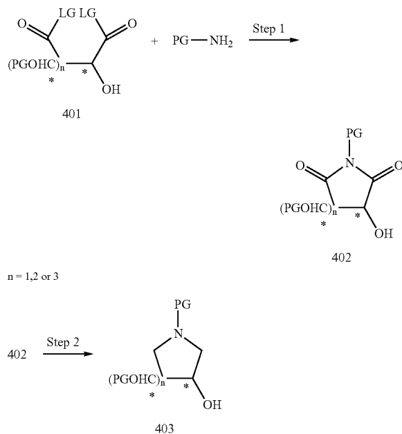
REACTION SCHEME 4
