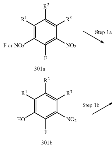
REACTION SCHEME 3
