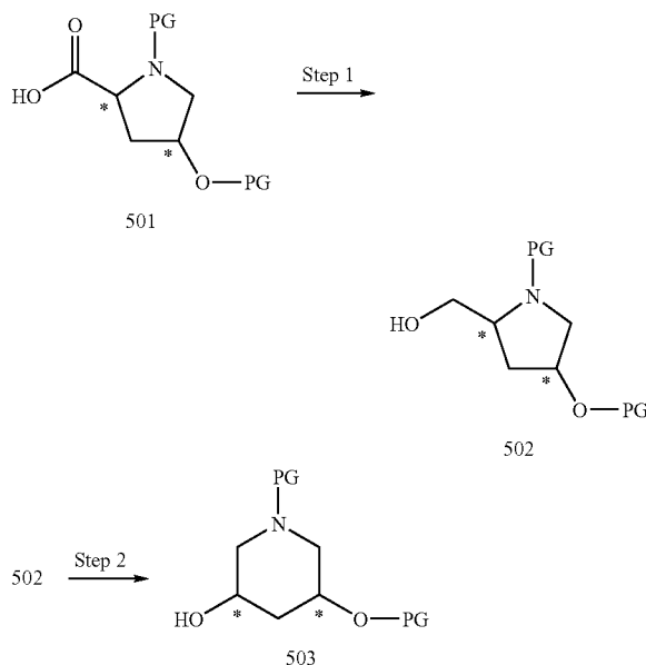
REACTION SCHEME 5
