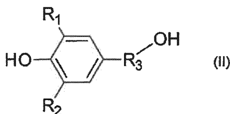
[Chemical Formula 4]
