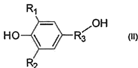
[Chemical Formula 2]
