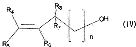
[Chemical Formula 7]
