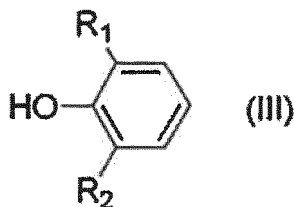
[Chemical Formula 6]
