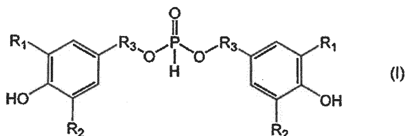
[Chemical Formula 3]
