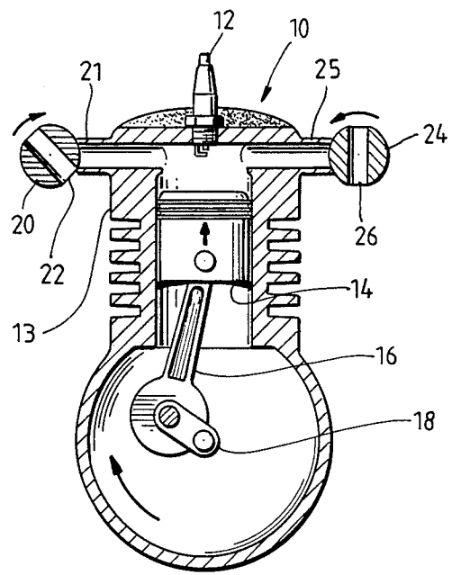
Fig. 2 (COMPRESSION STROKE)
