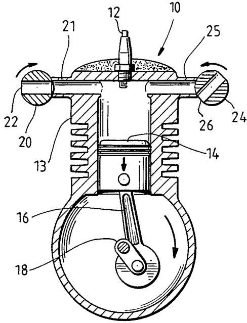
Fig. 1 (INTAKE STROKE)
