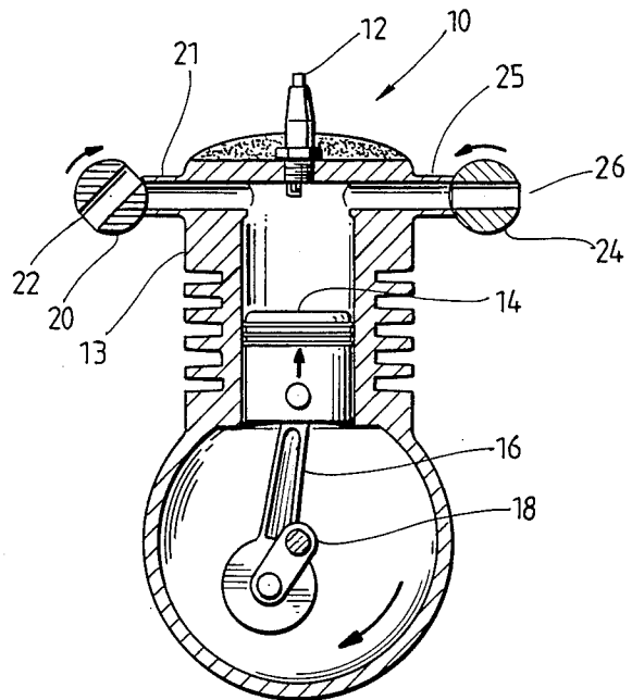
Fig. 4 (EXHAUST STROKE)
