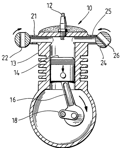
Fig. 3 (POWER STROKE)
