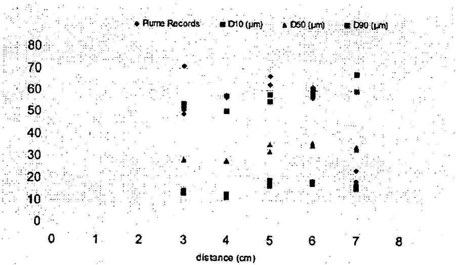
Figure 14: Device to Laser Beam Placement Results, Dv10, Dv50, Dv90 vs. Distance to Laser Beam
