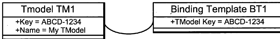
Primary & Foreign Keys
