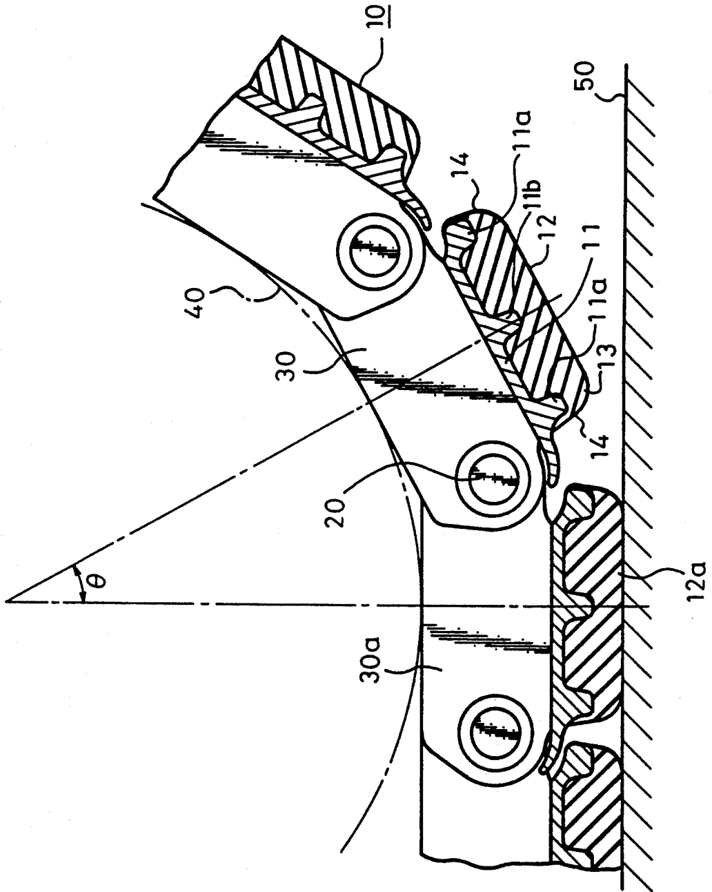
Fig. 4 (PRIOR ART)
