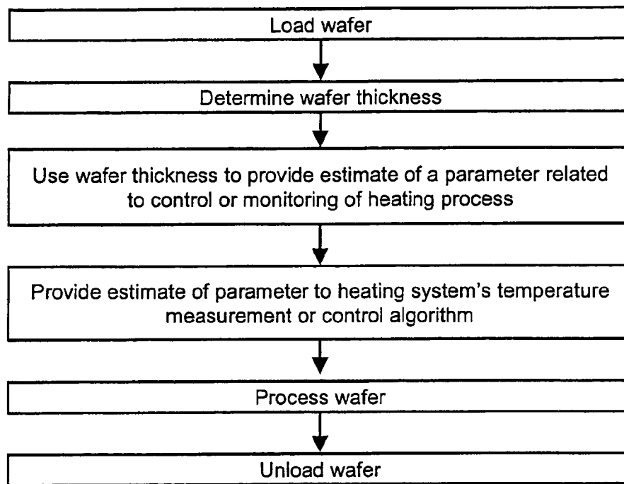
Example approach for using wafer thickness information to improve control or monitoring of a heating process.
