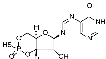
Rp-isomer
