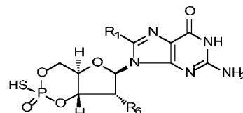
Rp-isomer,
