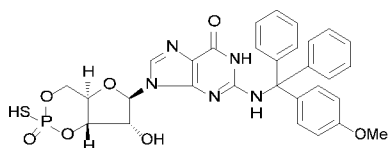
Rp-isomer
