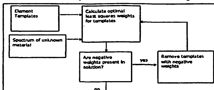
Iterative Least Squares Initialisation Block Diagram
