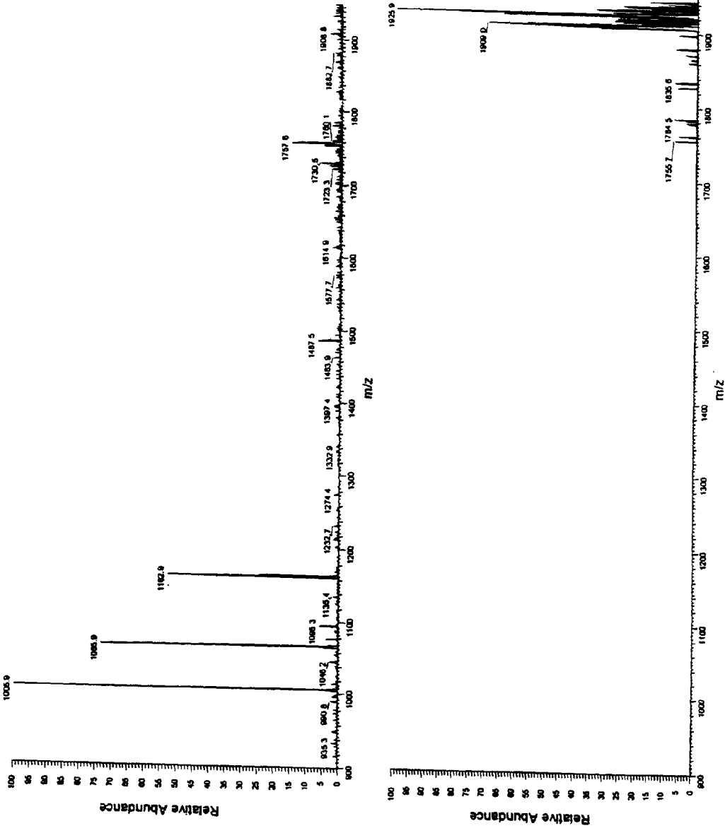
Figure 2. MS/MS of control RNA/DNA (upper); control+paromomycin (lower)
