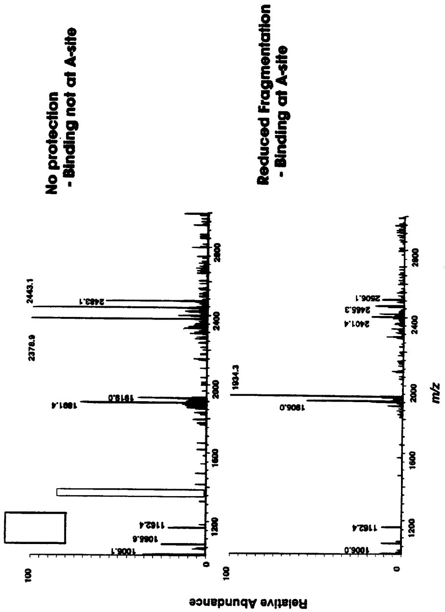
Figure 23 MASS Protection Assay
