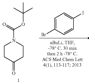
Scheme E6.
