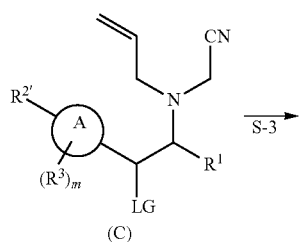
Scheme 2.
