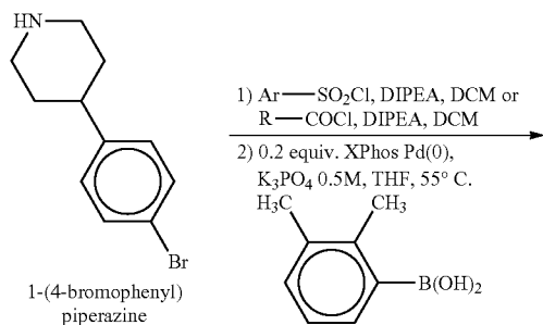
Scheme E5.
