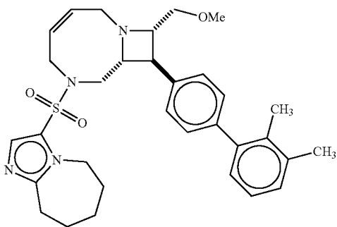
JP-S17-OMe
