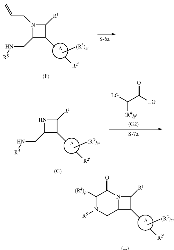
Scheme 3B.
