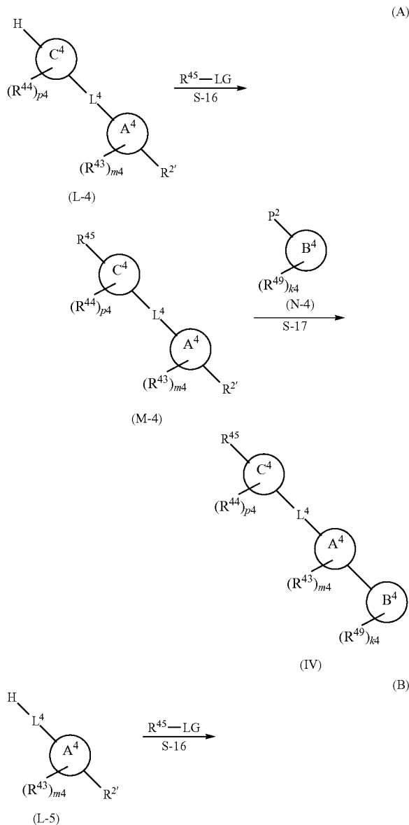
Scheme 10.
