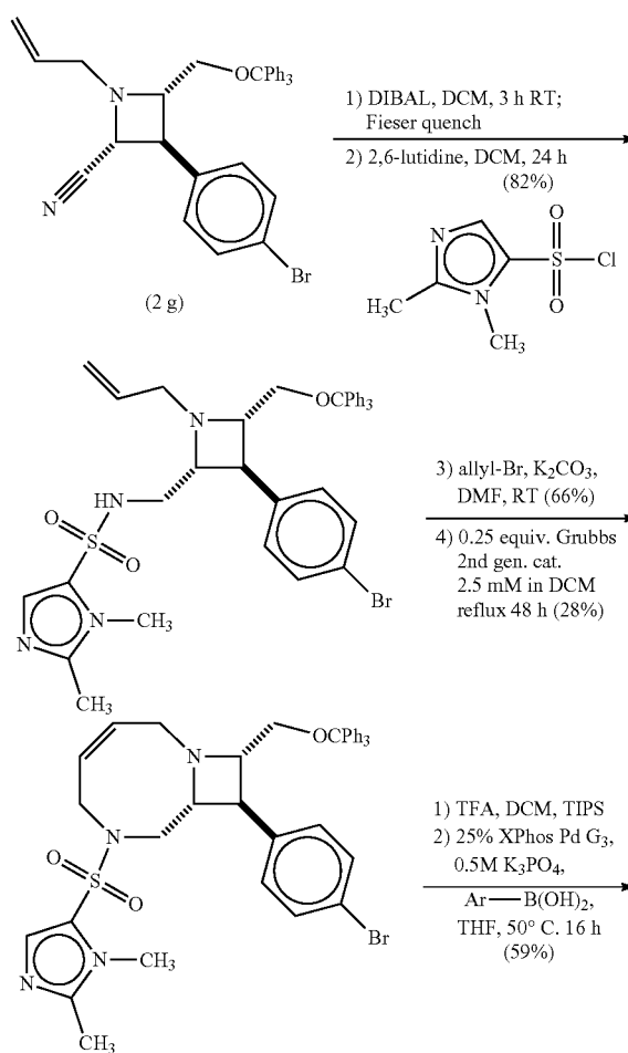
Scheme E4.
