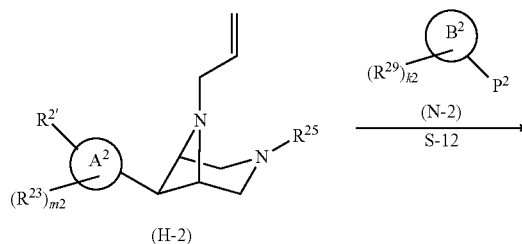
Scheme 8.
