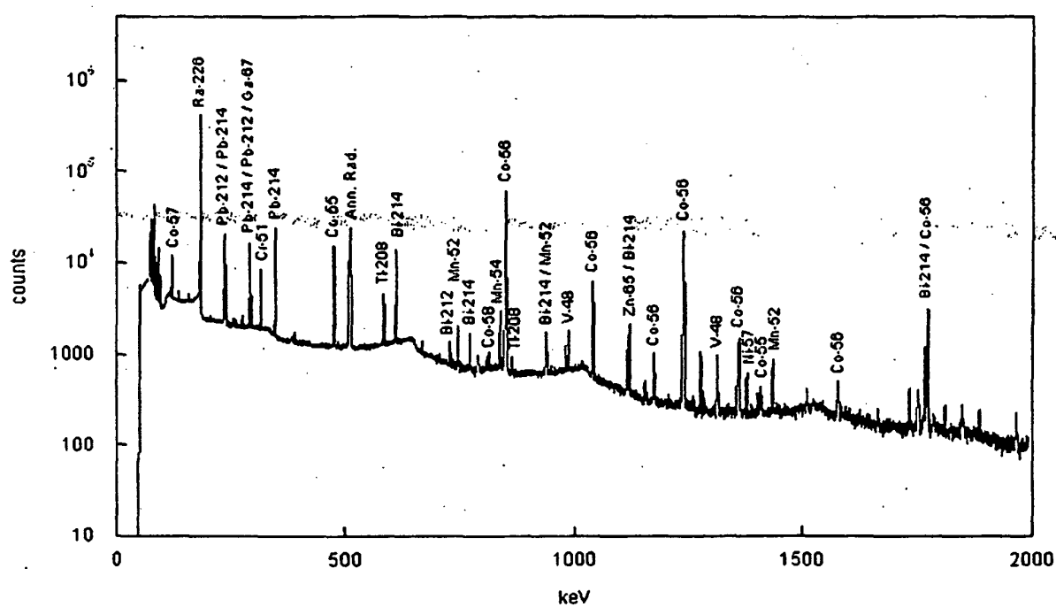
Fig.2a: \gamma -spectrum of the ^{226}\text{Ra} -fraction after the first Ra/Ac separation with RE Resin
