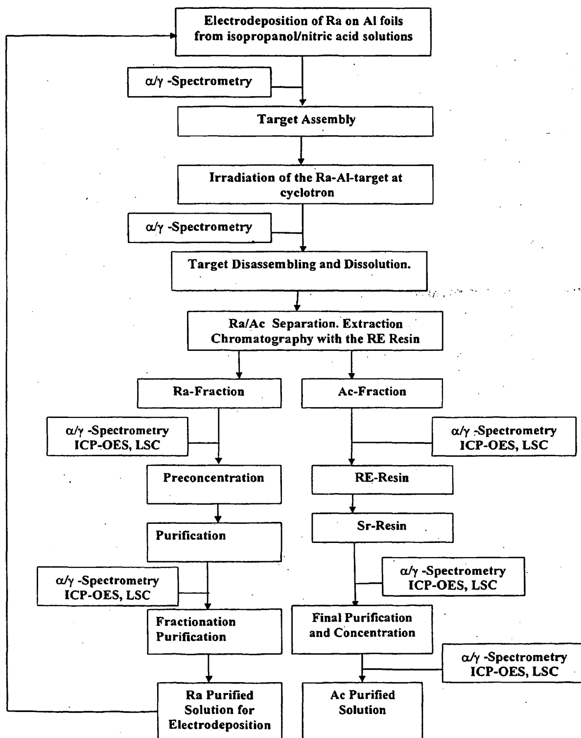
Fig.1. General Scheme for the Extraction of Ac from Ra/Al Irradiated Targets
