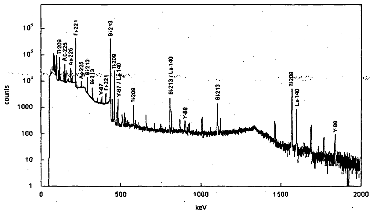
Fig.2b: \gamma -spectrum of the purified 225 Ac-fraction
