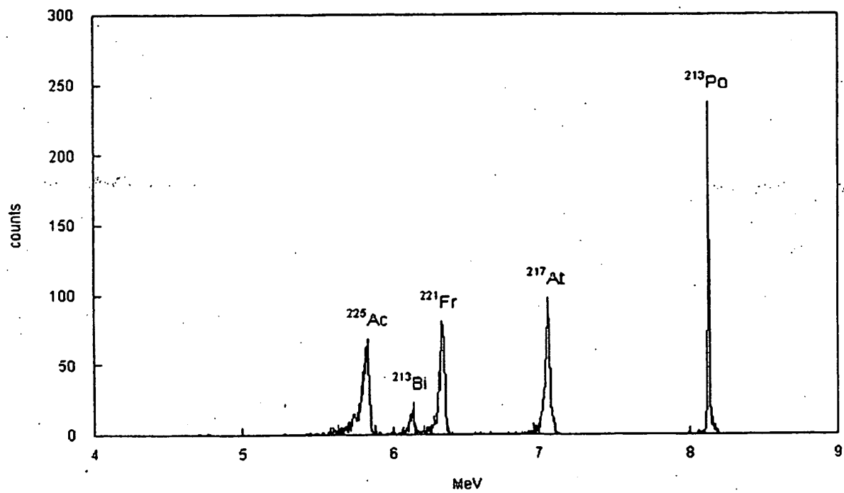
Fig.3b: \alpha -spectrum of ^{225}\text{Ac} after Po and Pb purification
