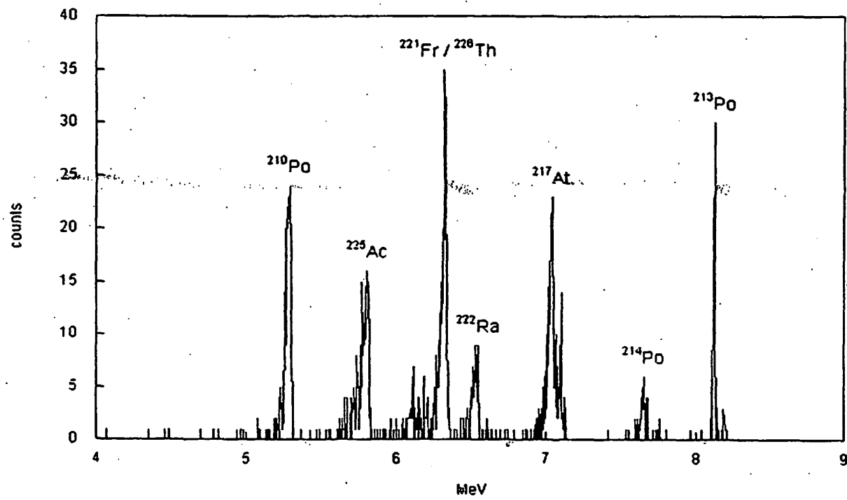
Fig.3a: \alpha -spectrum of ^{225}\text{Ac} before Po and Pb purification
