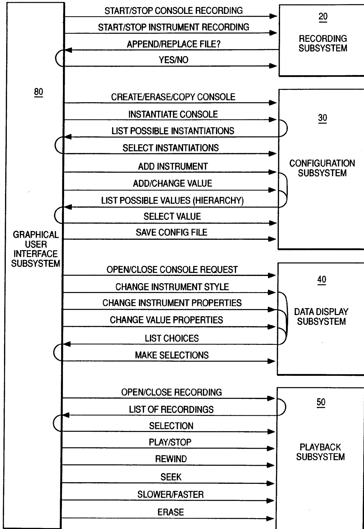
FIG. 21 GRAPHICAL USER INTERFACE SUBSYSTEM
