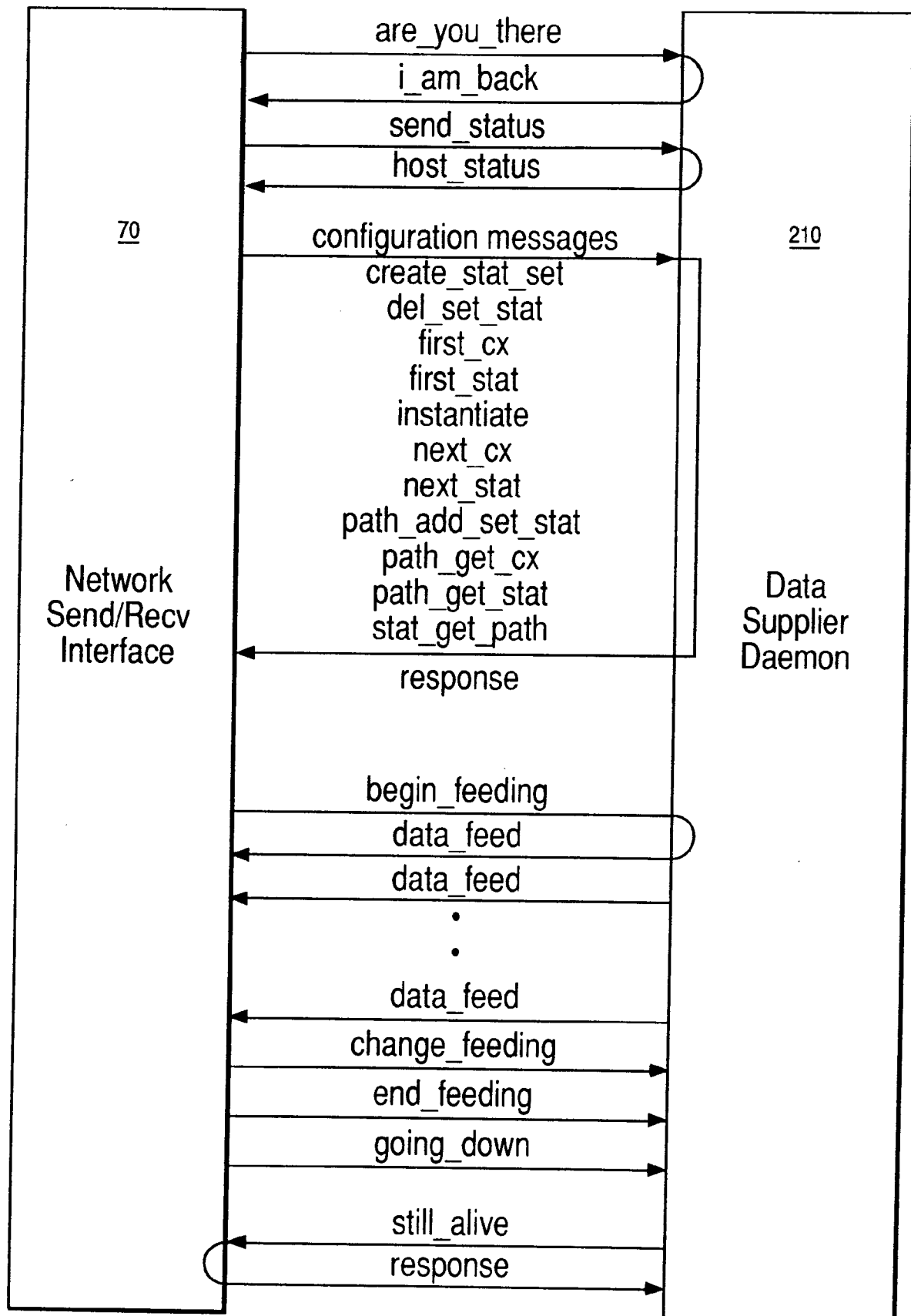
FIG. 25 DATA SUPPLIER DAEMON
