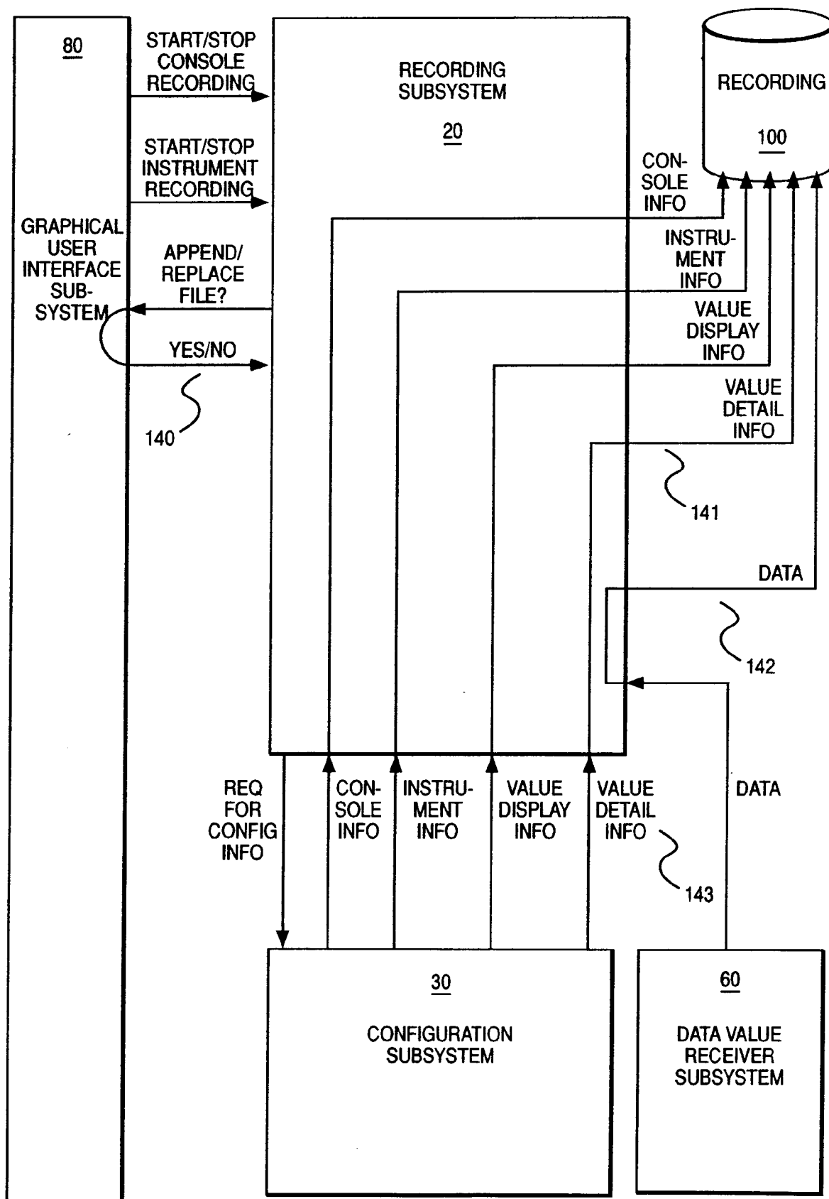
FIG. 10 RECORDING SUBSYSTEM
