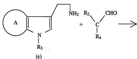
Scheme III
