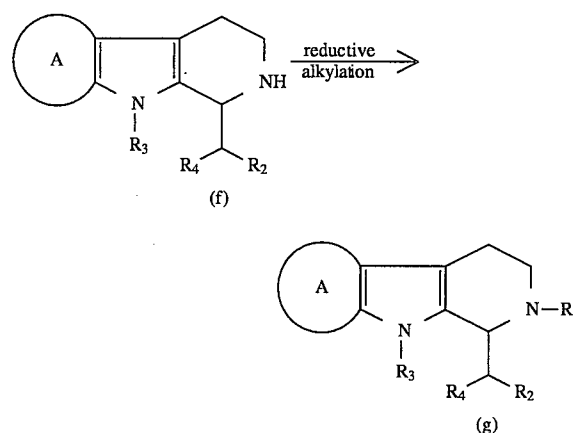
Scheme IV
