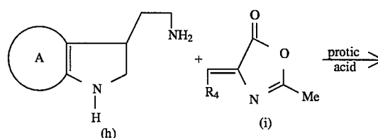
Scheme V
