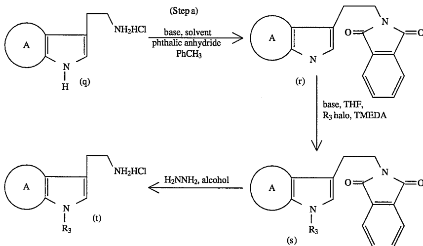
Scheme VII
