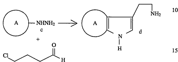
Scheme II
