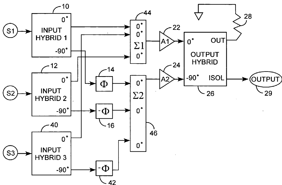
THREE SIGNAL INTERMODULATION CANCELLATION AMPLIFIER
