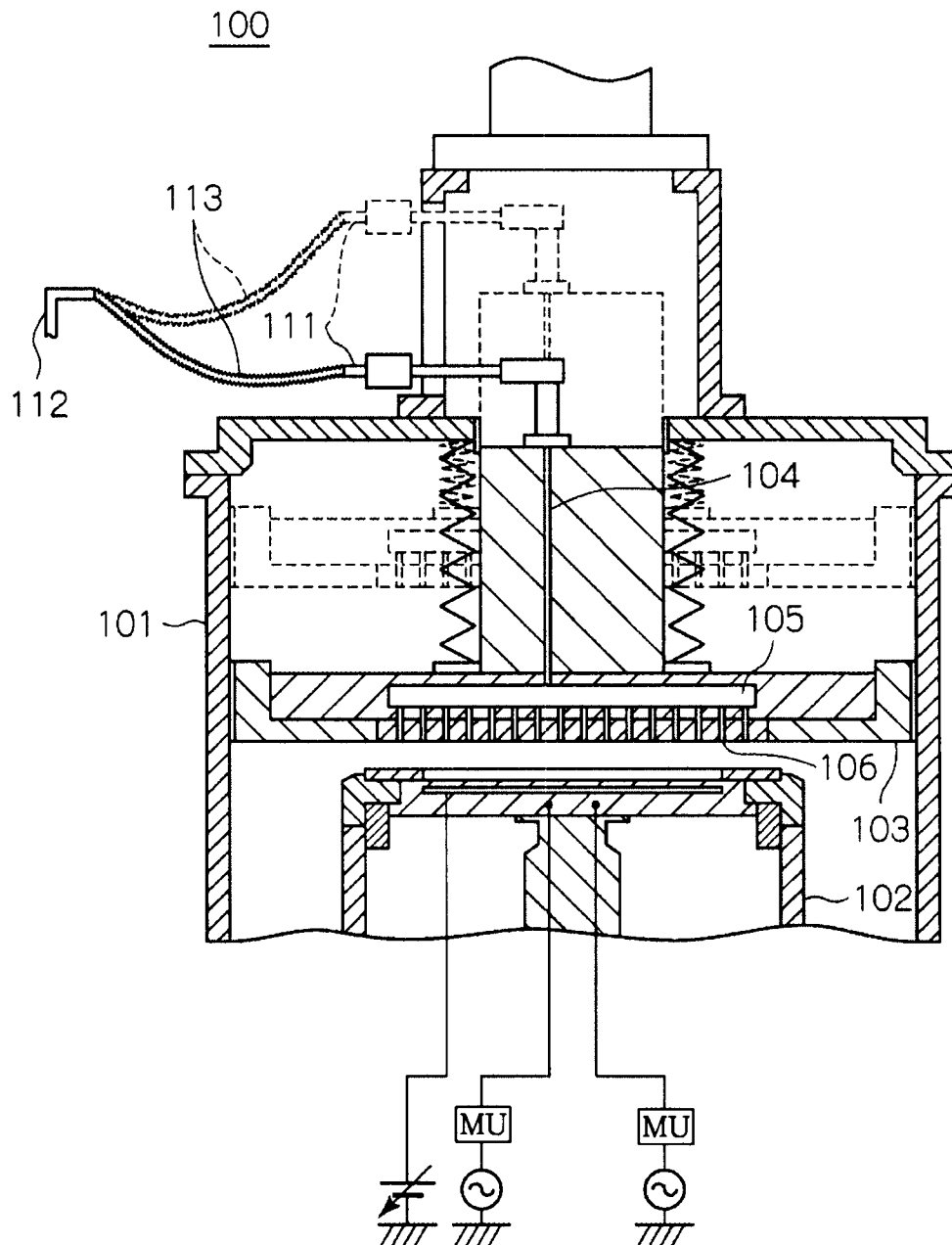
FIG. 6 (PRIOR ART)
