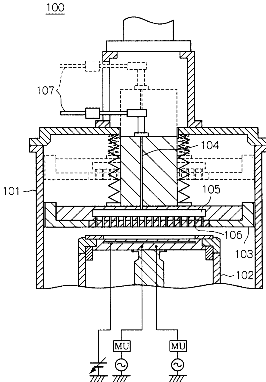
FIG. 4 (PRIOR ART)
