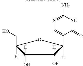
Pseudoisocytidine (psi ICR)
