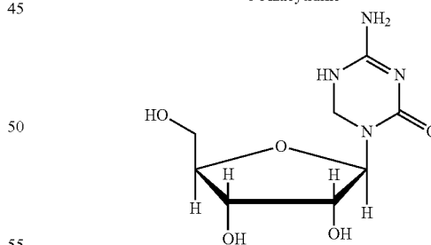
5-6-Dihydro-5-azacytidine
