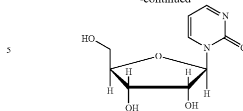
Zebularine
