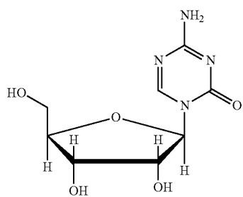
Azacitidine
