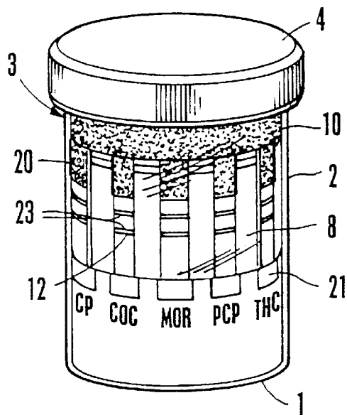
Fig. 1 EXISTING DEVICE
