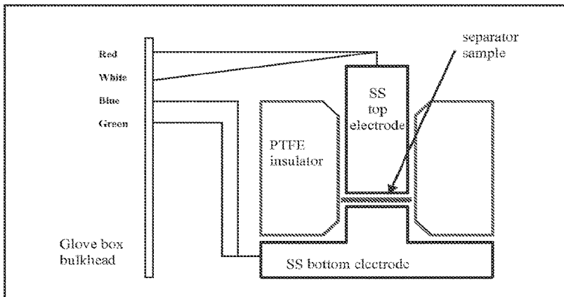
Fig. 6 Stainless steel fixture for electrical resistance measurement.
