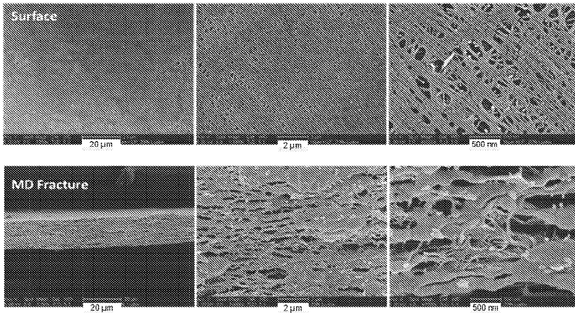
Fig. 5 Scanning electron micrographs of the surface and bulk structure of the separator dip coated through a 20% colloidal silica solution. The colloidal silica particles in the bulk were confirmed with energy dispersive x-ray analysis. The silica particles are the bright white spots in the highest magnification MD fracture photograph.
