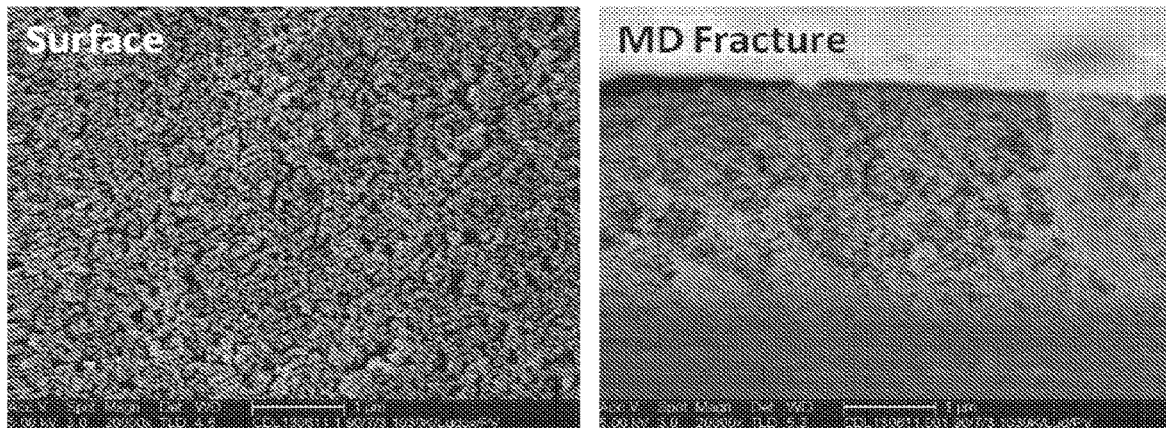
Fig. 8 SEM images of silica-coated separator from Example 9.
