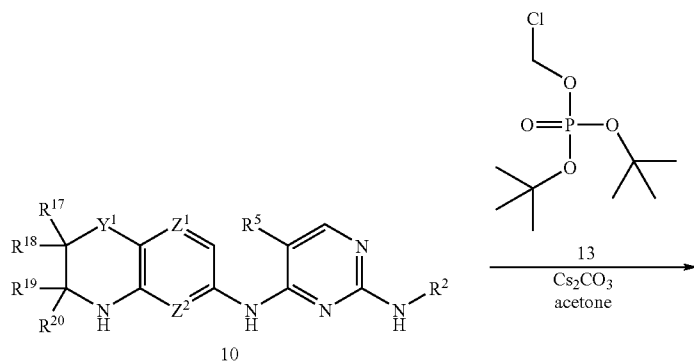
Scheme II
