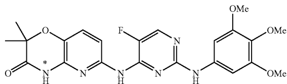
Compound 1
