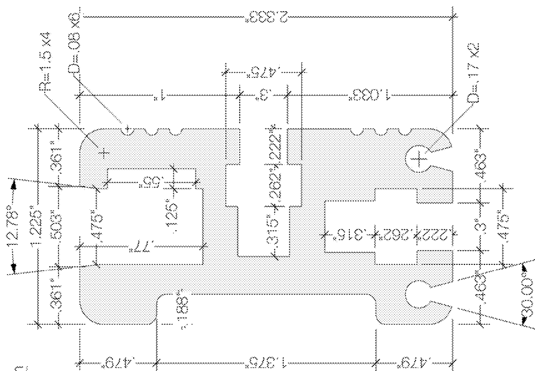
Truss Mount Custom Extrusion
