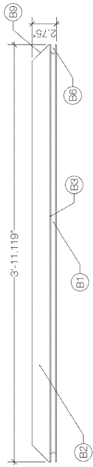
Fig. 6 Stage Mount Prototype Extrusion Top View Scale: 2" = 1'-0"
