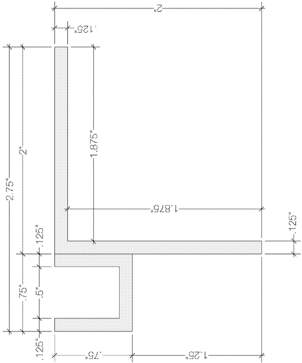
Fig. 4 Stage Mount Prototype Extrusion Scale: 2X
