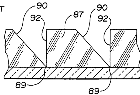
Fig. 13 PRIOR ART
