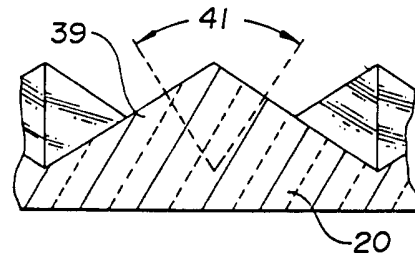
Fig.5 PRIOR ART
