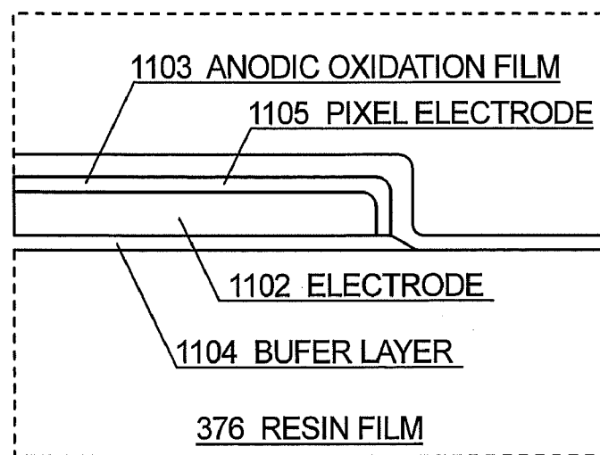
SCHEMATIC DIAGRAM OF ENLARGED ELECTRODE EDGE PORTION
