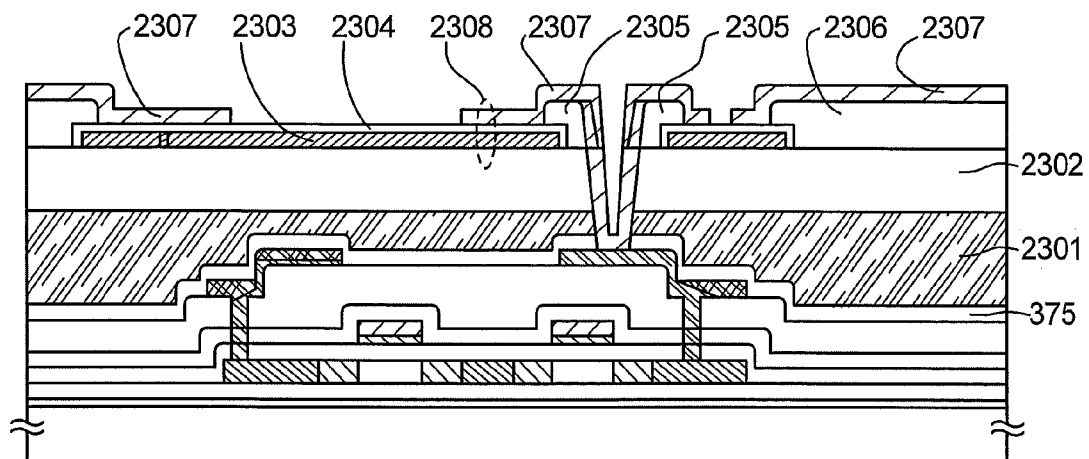
701: n-CHANNEL TFT
