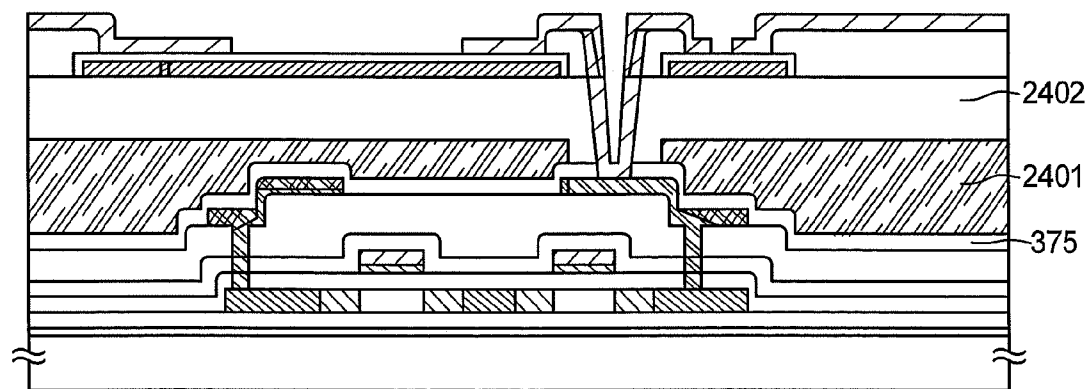
701: n-CHANNEL TFT
