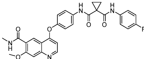
Compound 1
