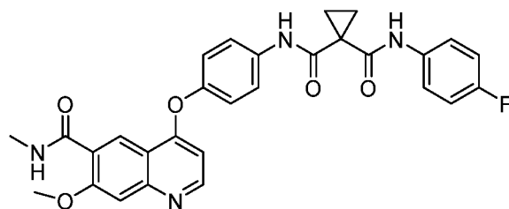
Compound 1
