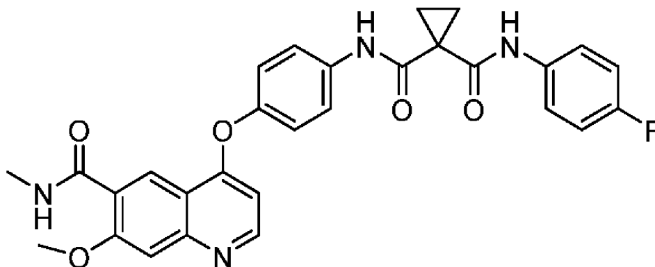
Compound 1
