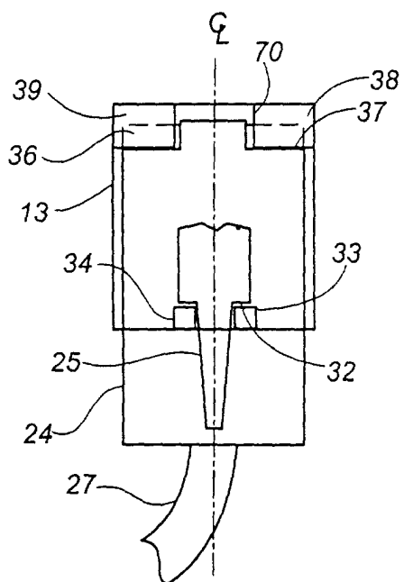
FIG. 6 (PRIOR ART)
