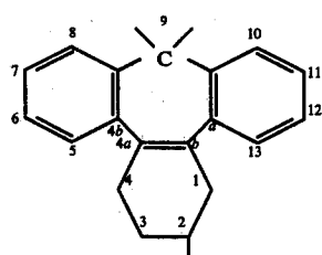
1,2,3,4-tetrahydro-9H-tribenzo(b,d,f)-cycloheptatriene
