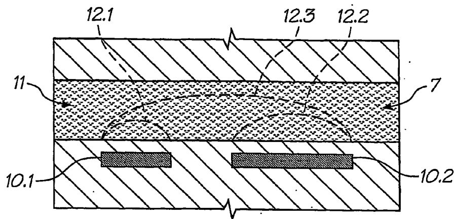
FIG. 52 (PRIOR ART)
