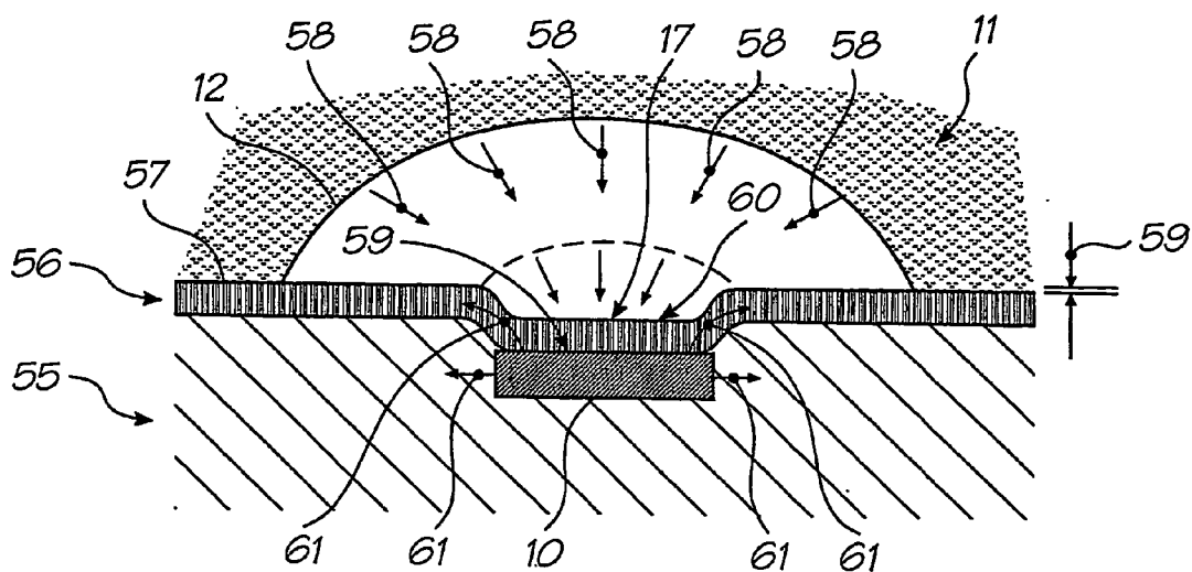
FIG. 47 (PRIOR ART)
