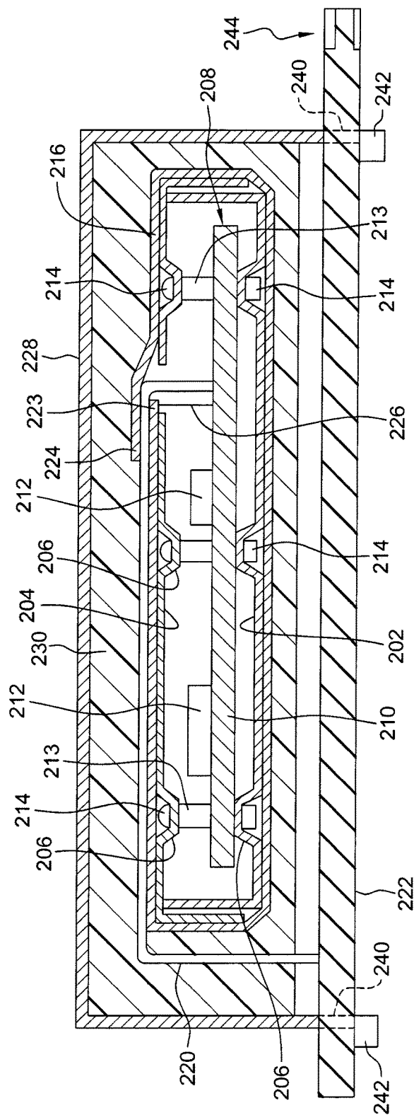
FIG. 2 (PRIOR ART)
